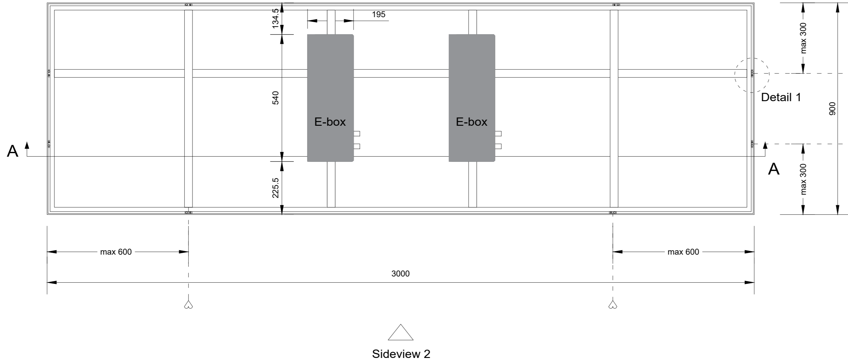
Backview (1:10)
