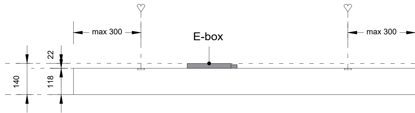
Section A-A (1:10)
