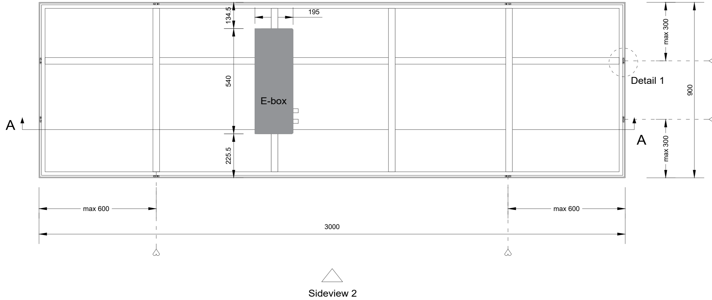
Backview (1:10)
