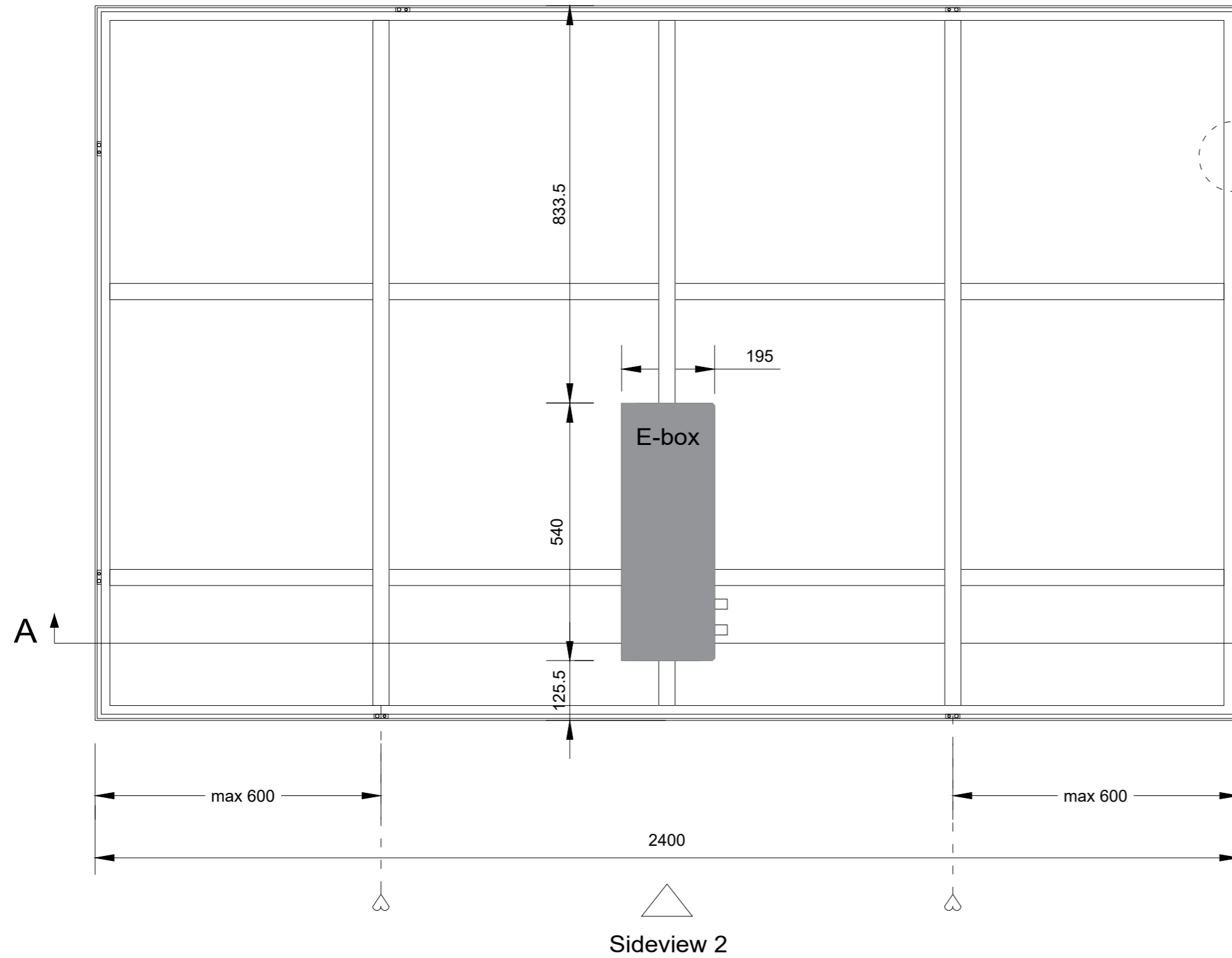
Backview (1:10)
