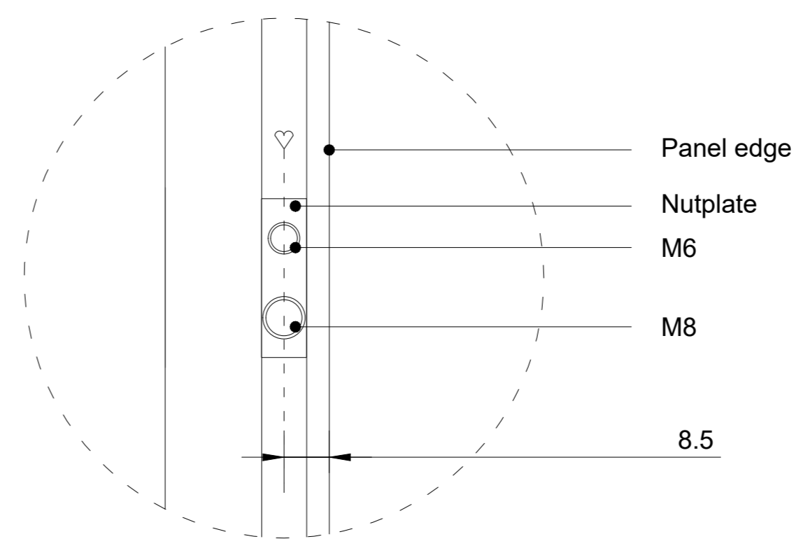
Detail 1 (1:1)
