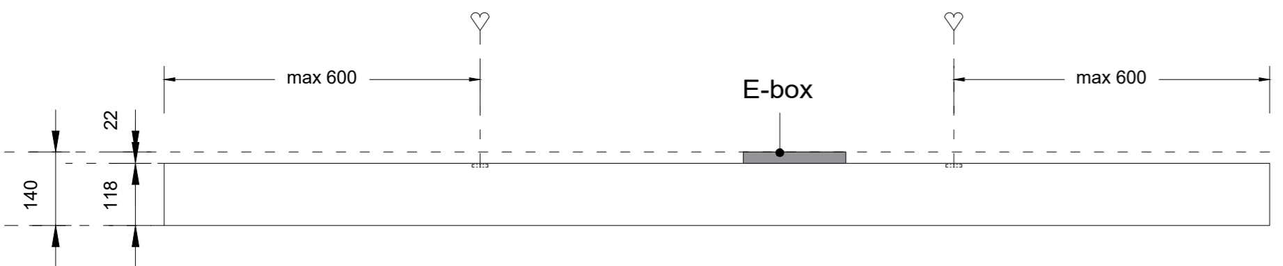
Sideview 2 - mounting position (1:10)
