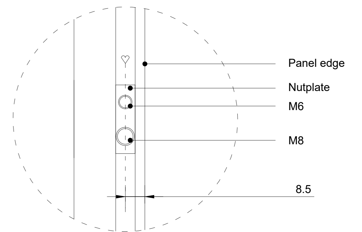
Detail 1 (1:1)
