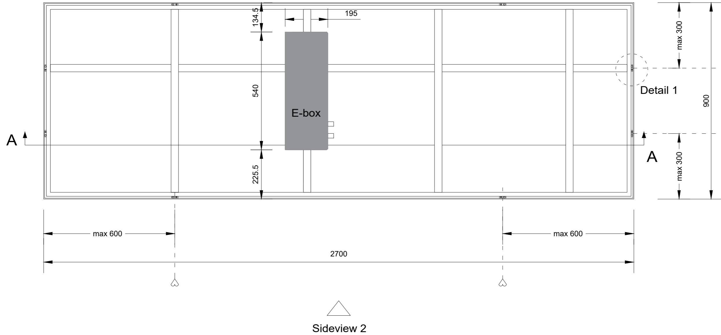
Backview (1:10)
