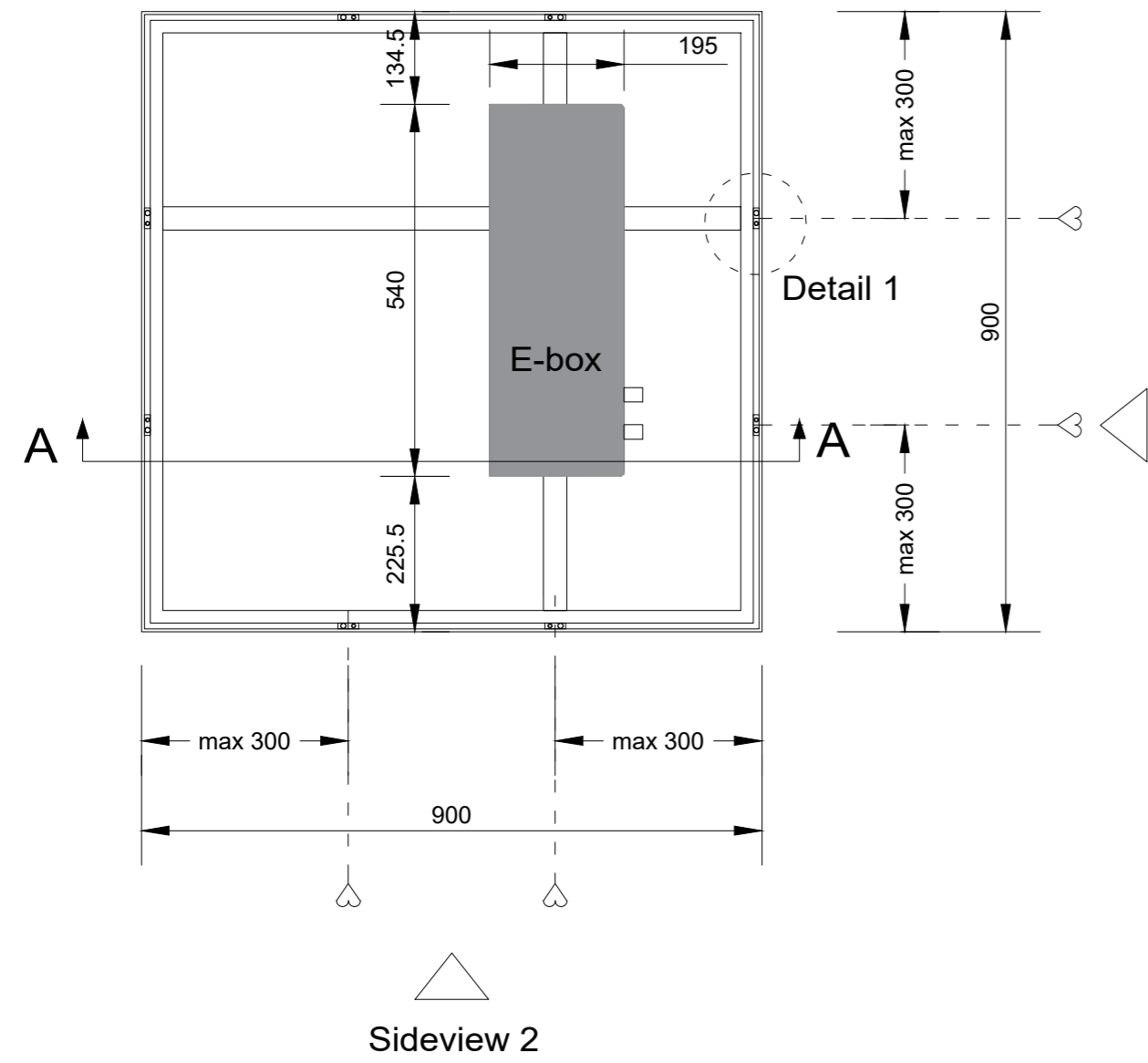
Backview (1:10)
