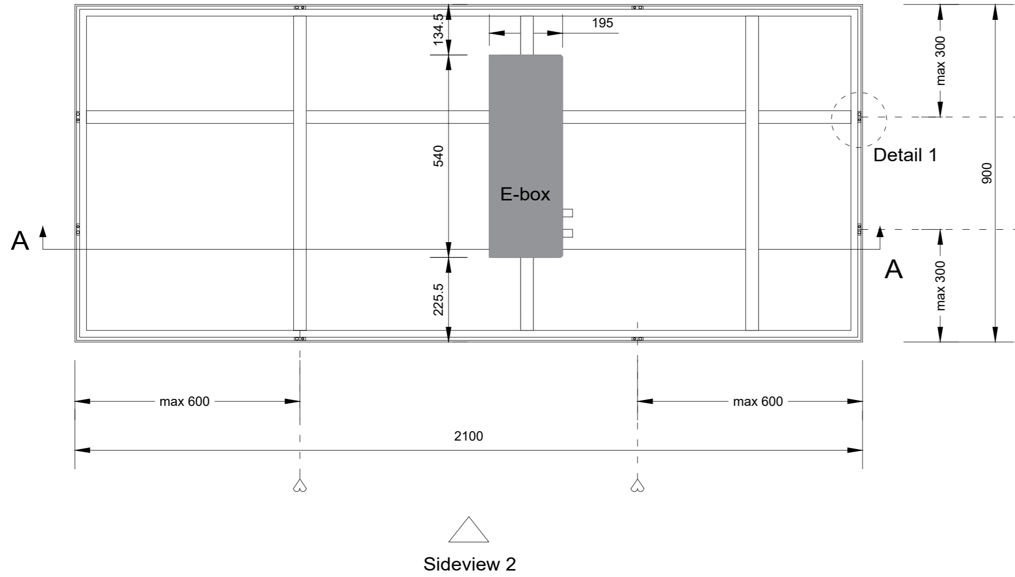
Backview (1:10)
