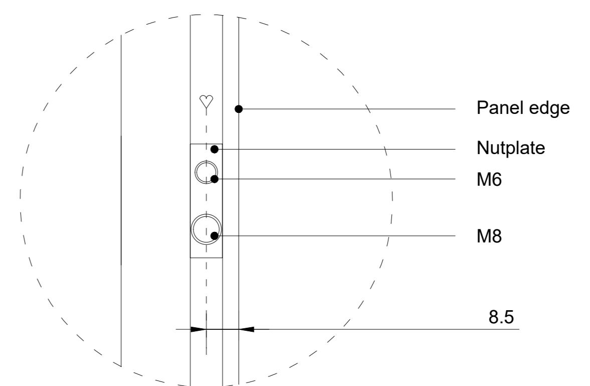
Detail 1 (1:1)
