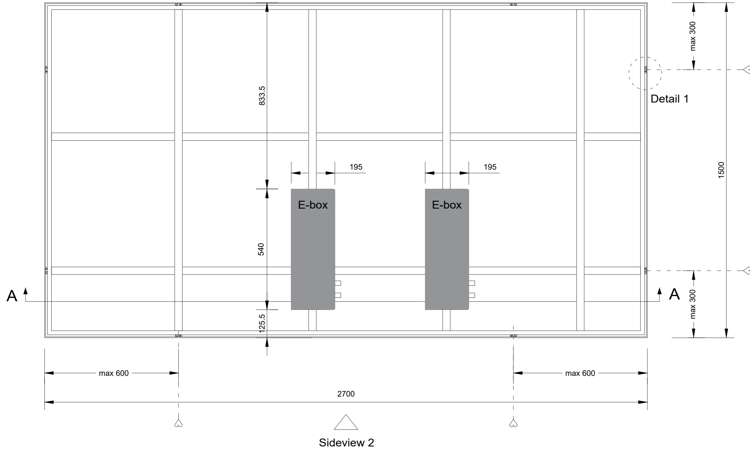
Backview (1:10)
