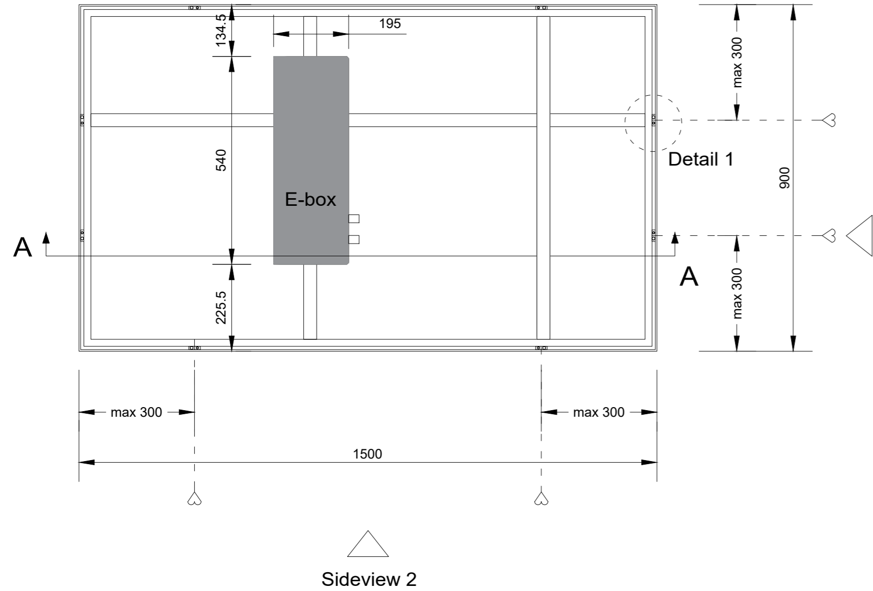
Backview (1:10)
