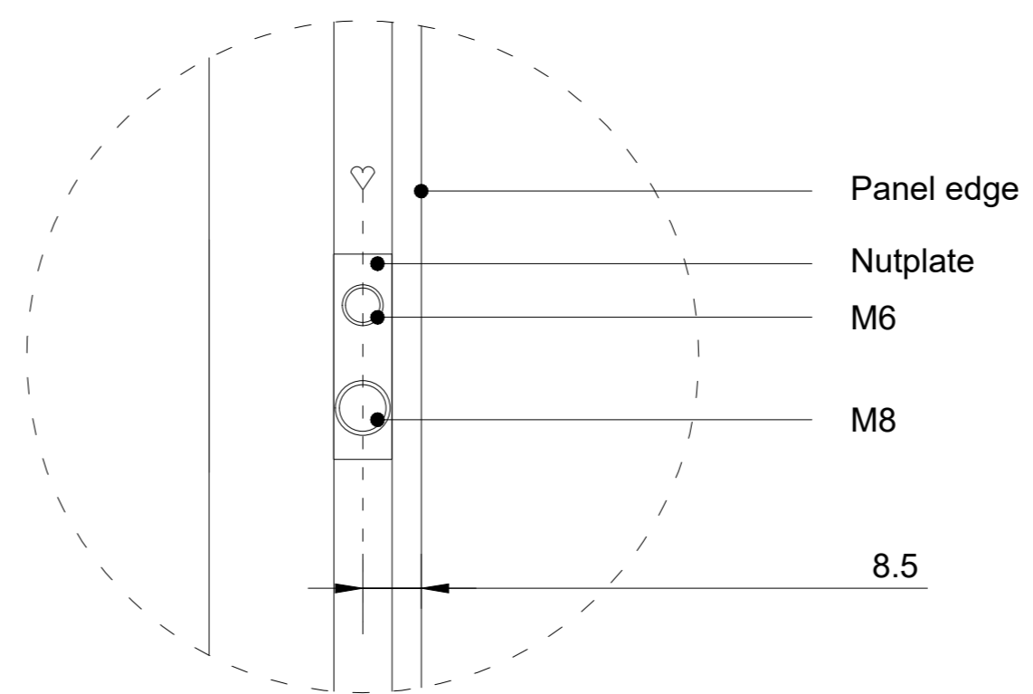
Detail 1 (1:1)
