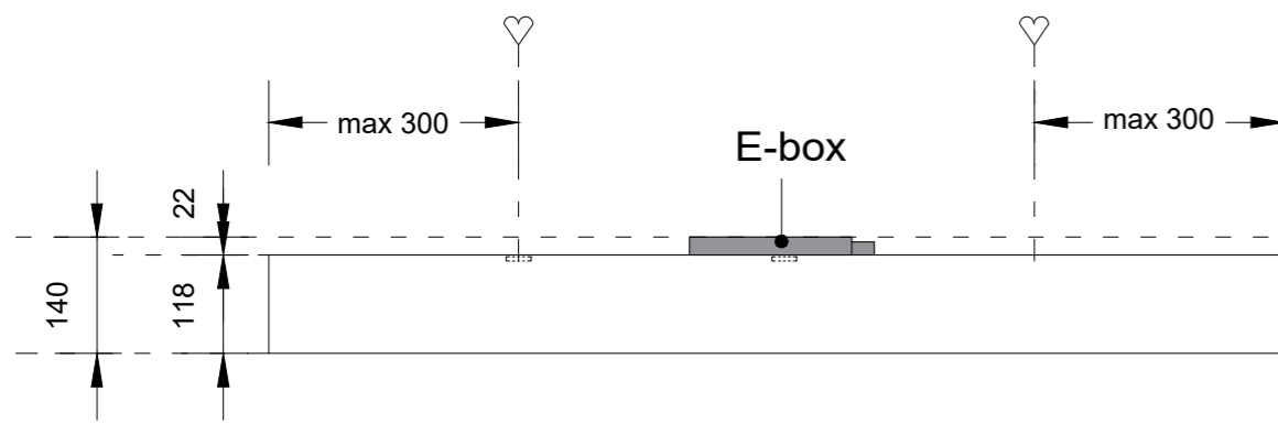
Sideview 2 - mounting position (1:10)
