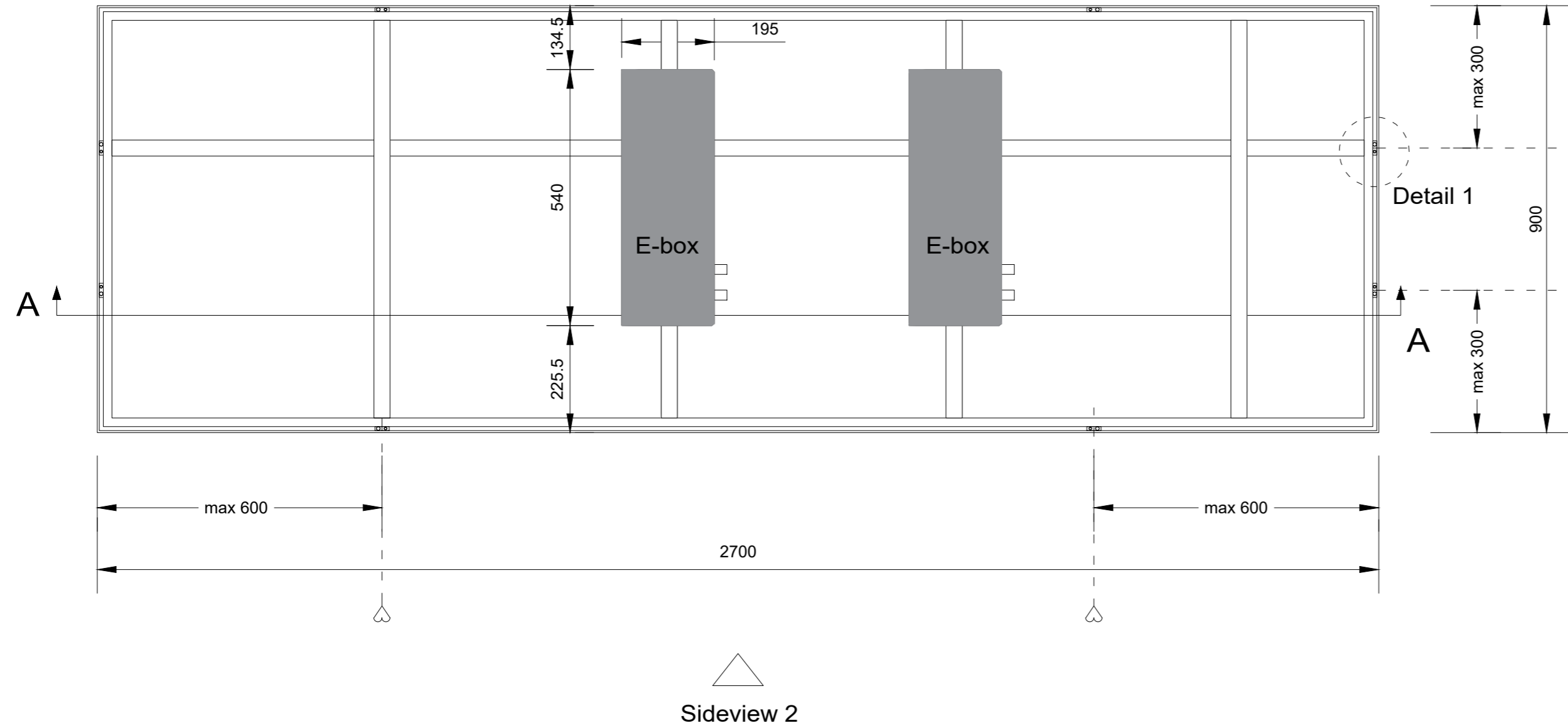
Backview (1:10)
