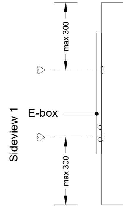
Sideview 1 - mounting position (1:10)
