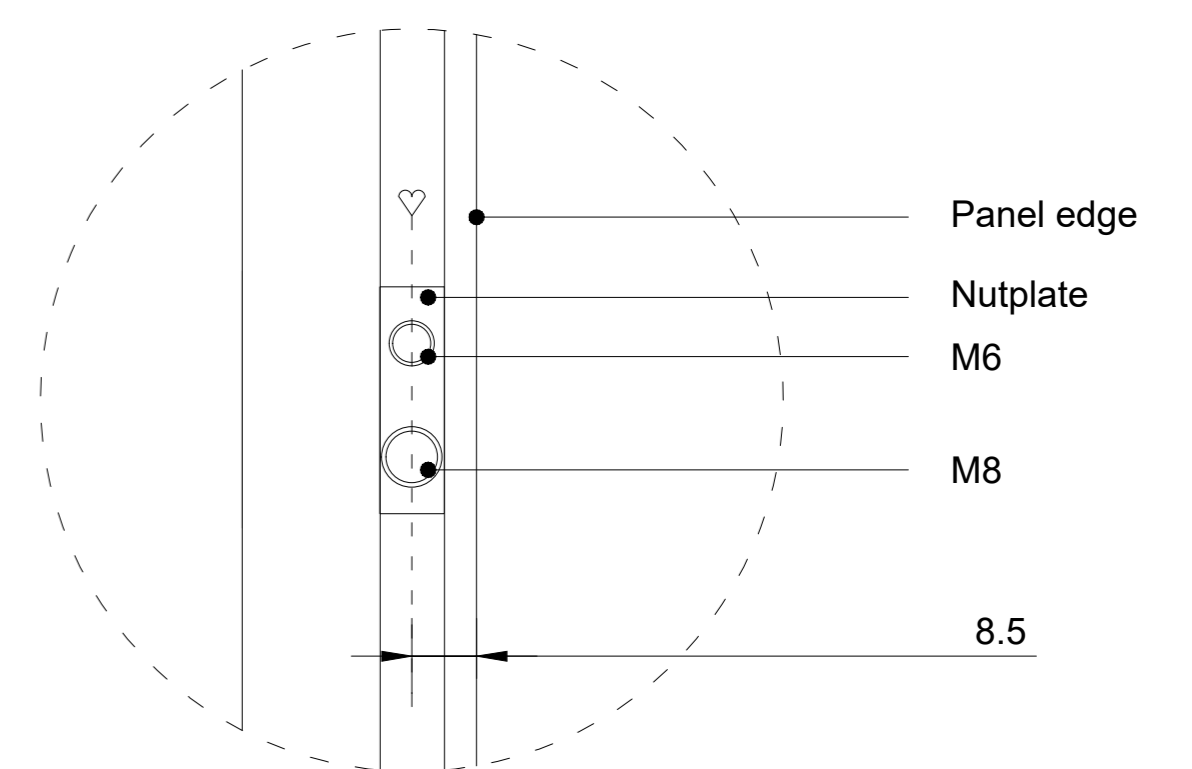
Detail 1 (1:1)
