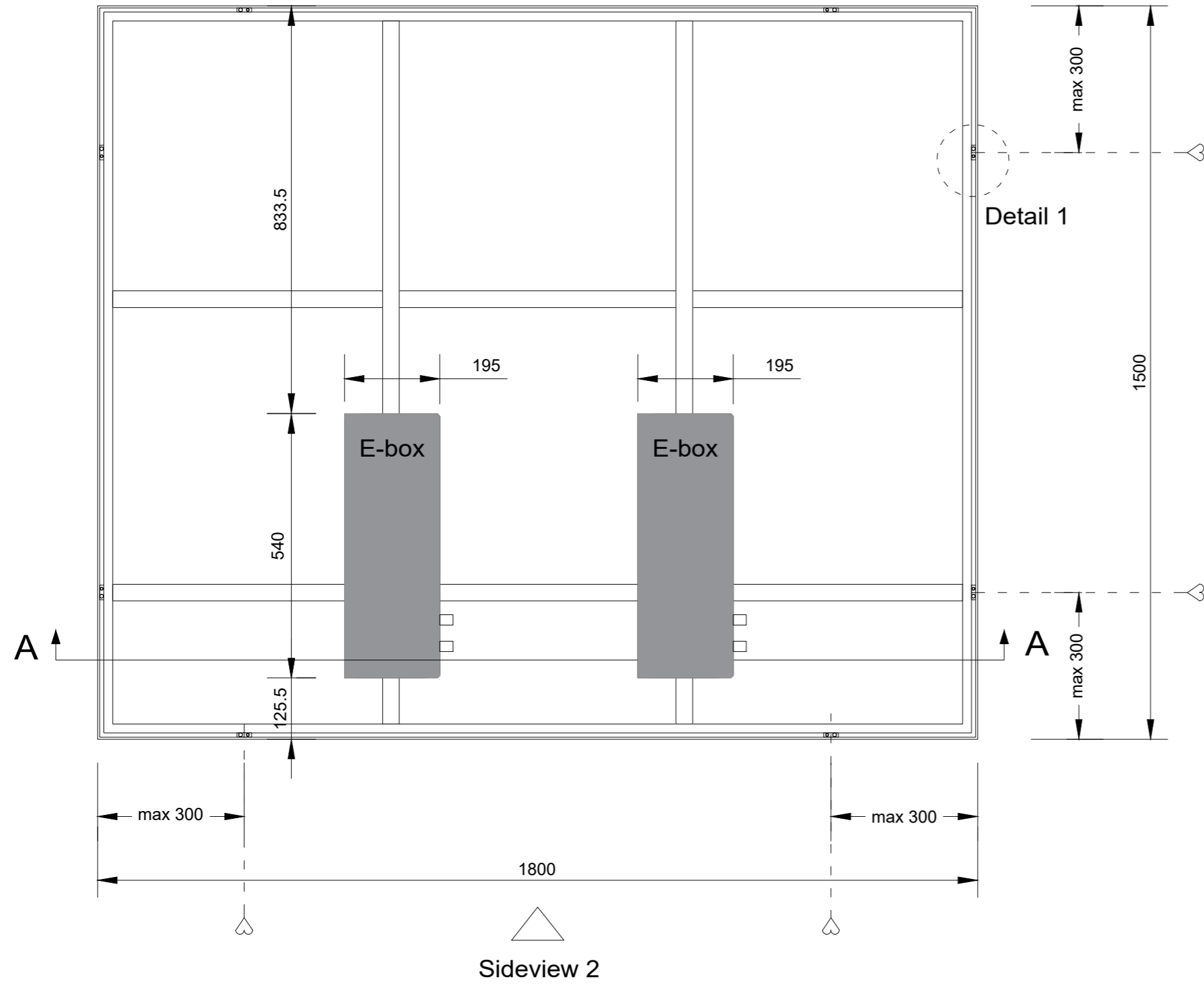
Backview (1:10)
