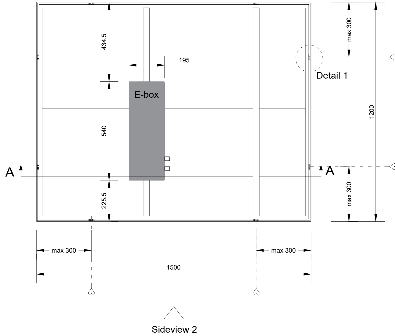
Backview (1:10)
