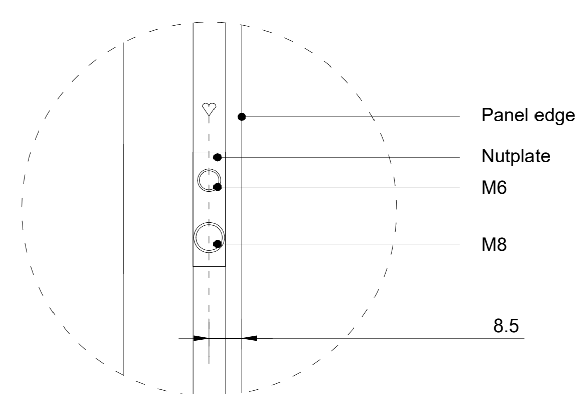
Detail 1 (1:1)
