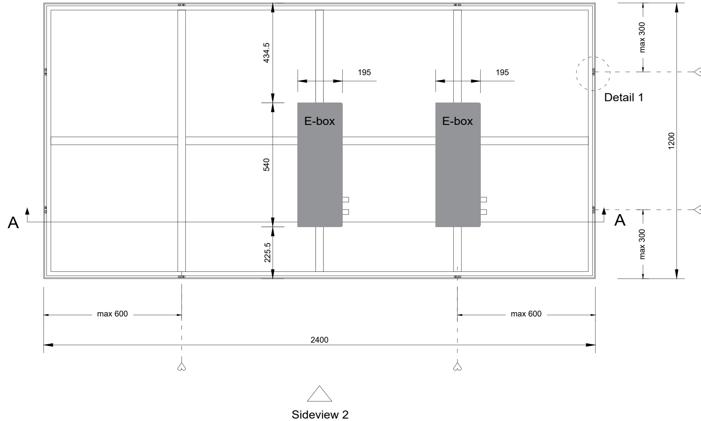
Backview (1:10)
