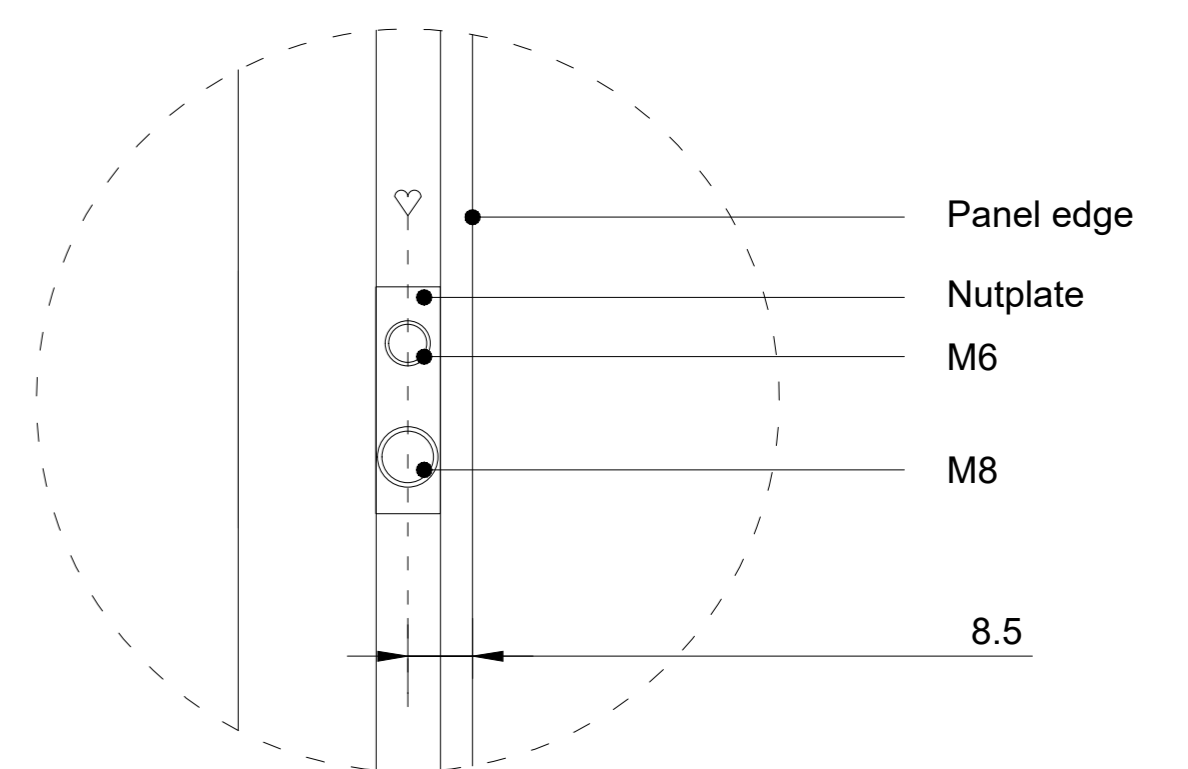
Detail 1 (1:1)
