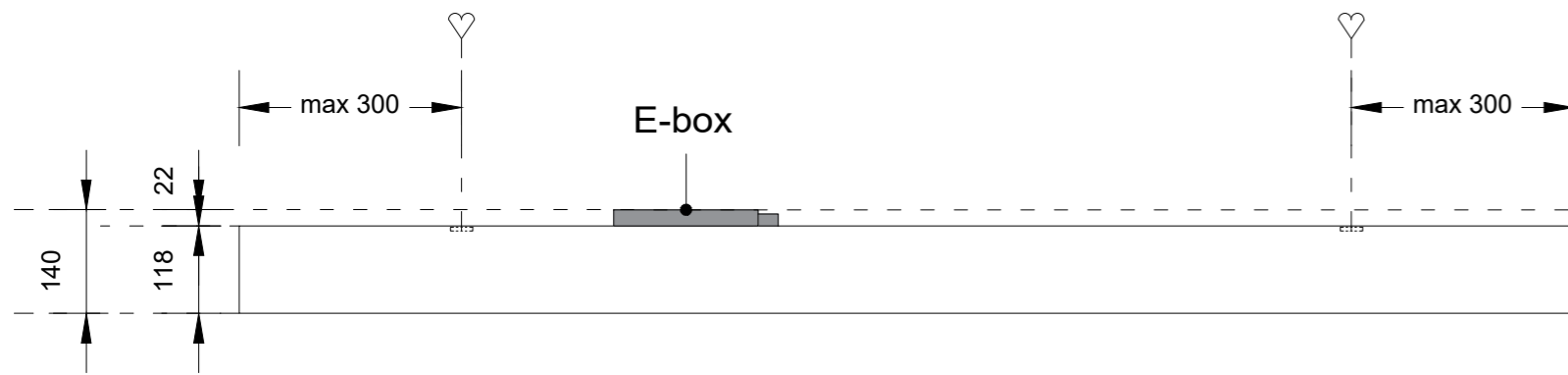
Section A-A (1:10)
