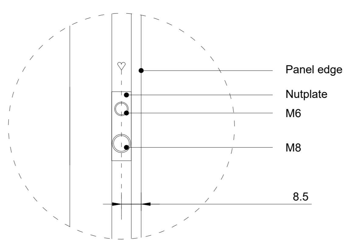
Detail 1 (1:1)
