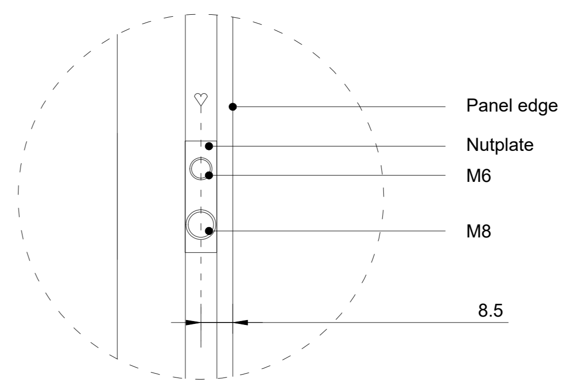
Detail 1 (1:1)
