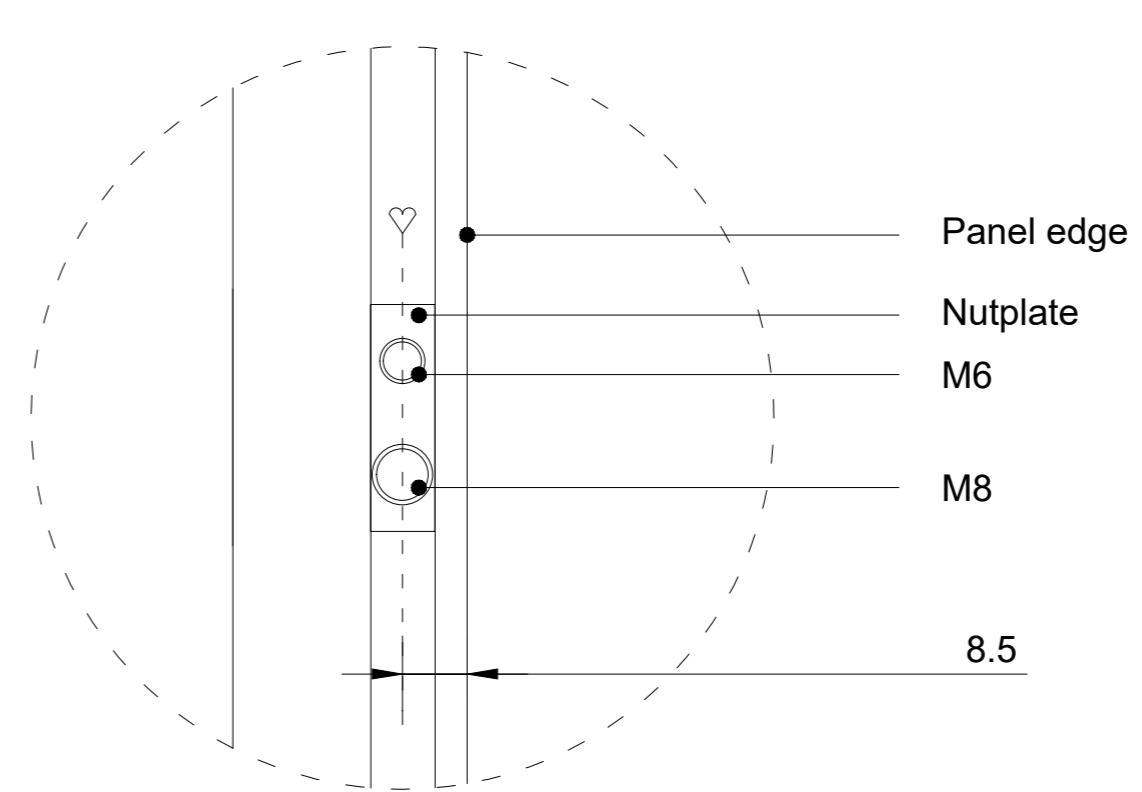
Detail 1 (1:1)
