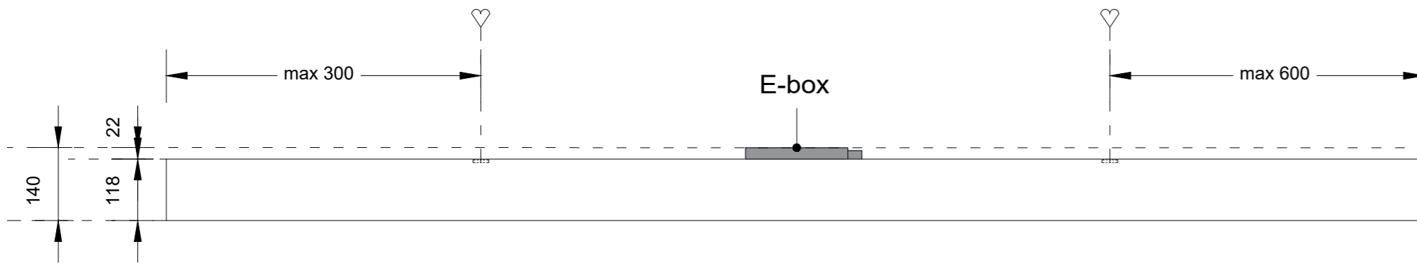
Section A-A (1:10)
