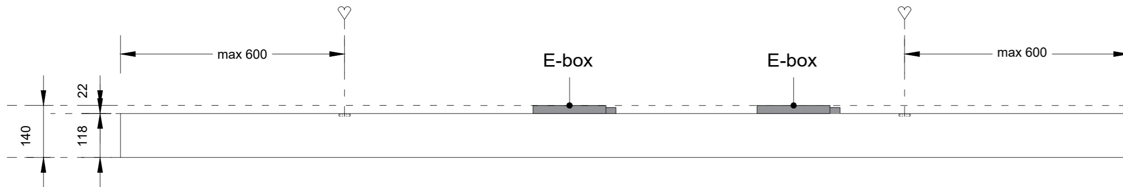
Section A-A (1:10)
