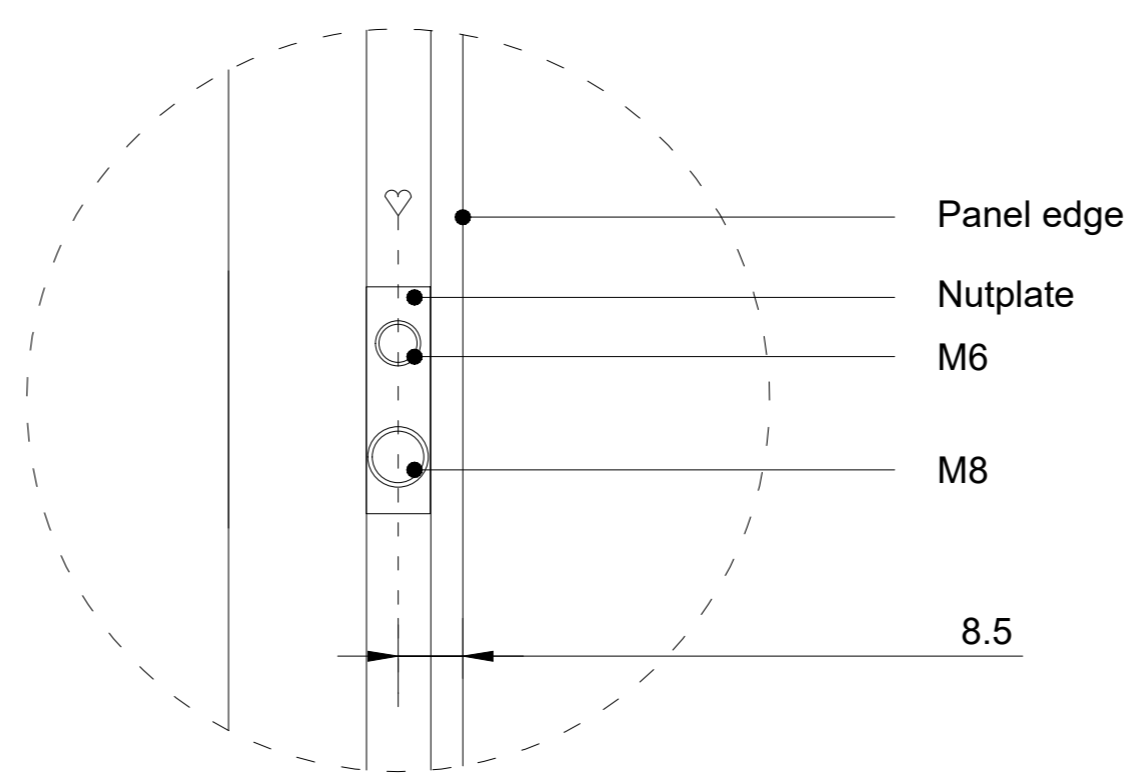
Detail 1 (1:1)
