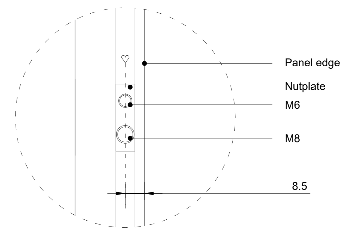
Detail 1 (1:1)
