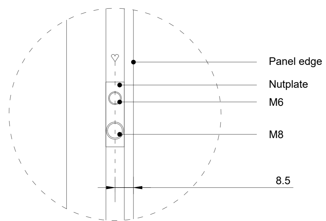
Detail 1 (1:1)
