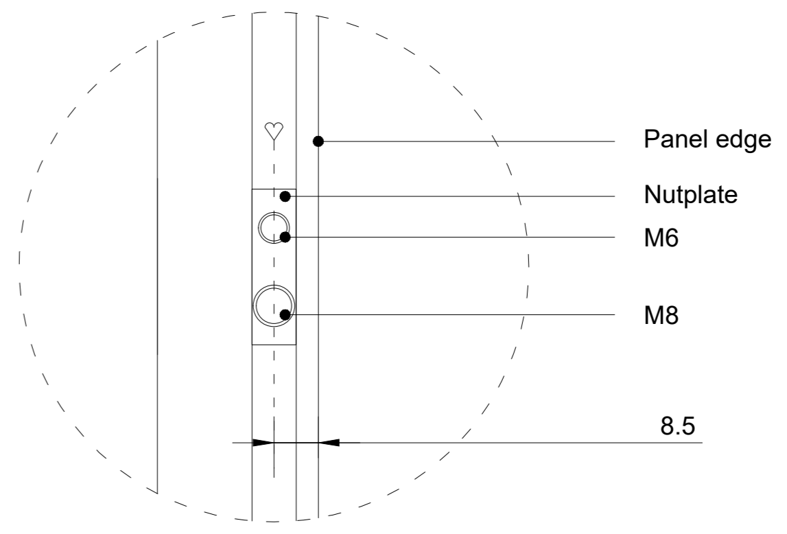
Detail 1 (1:1)
