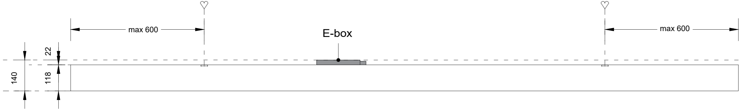
Section A-A (1:10)
