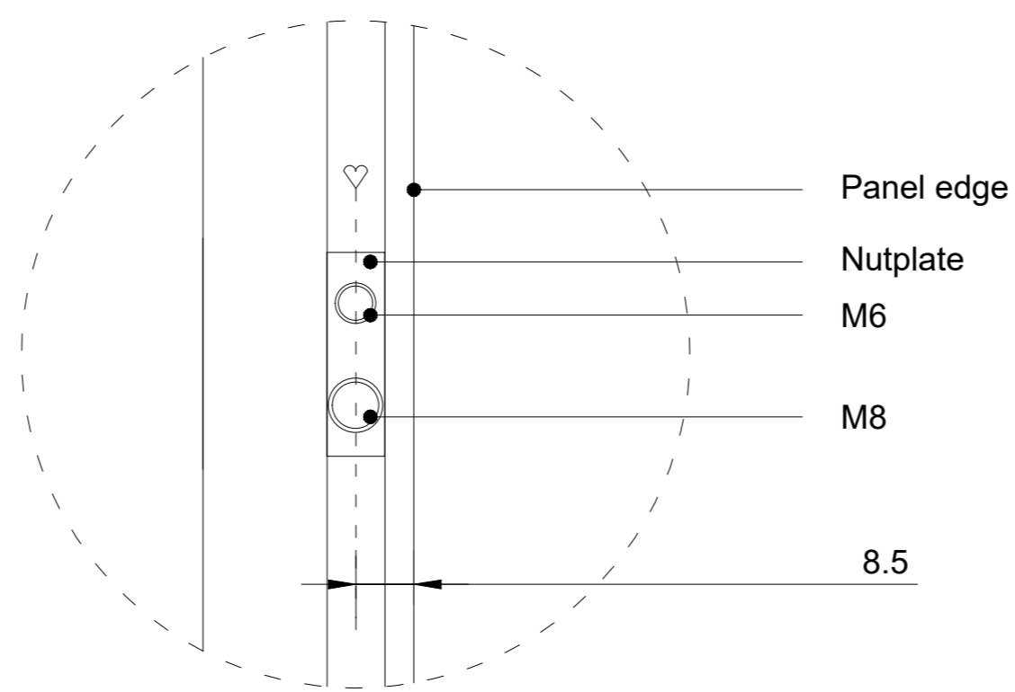
Detail 1 (1:1)
