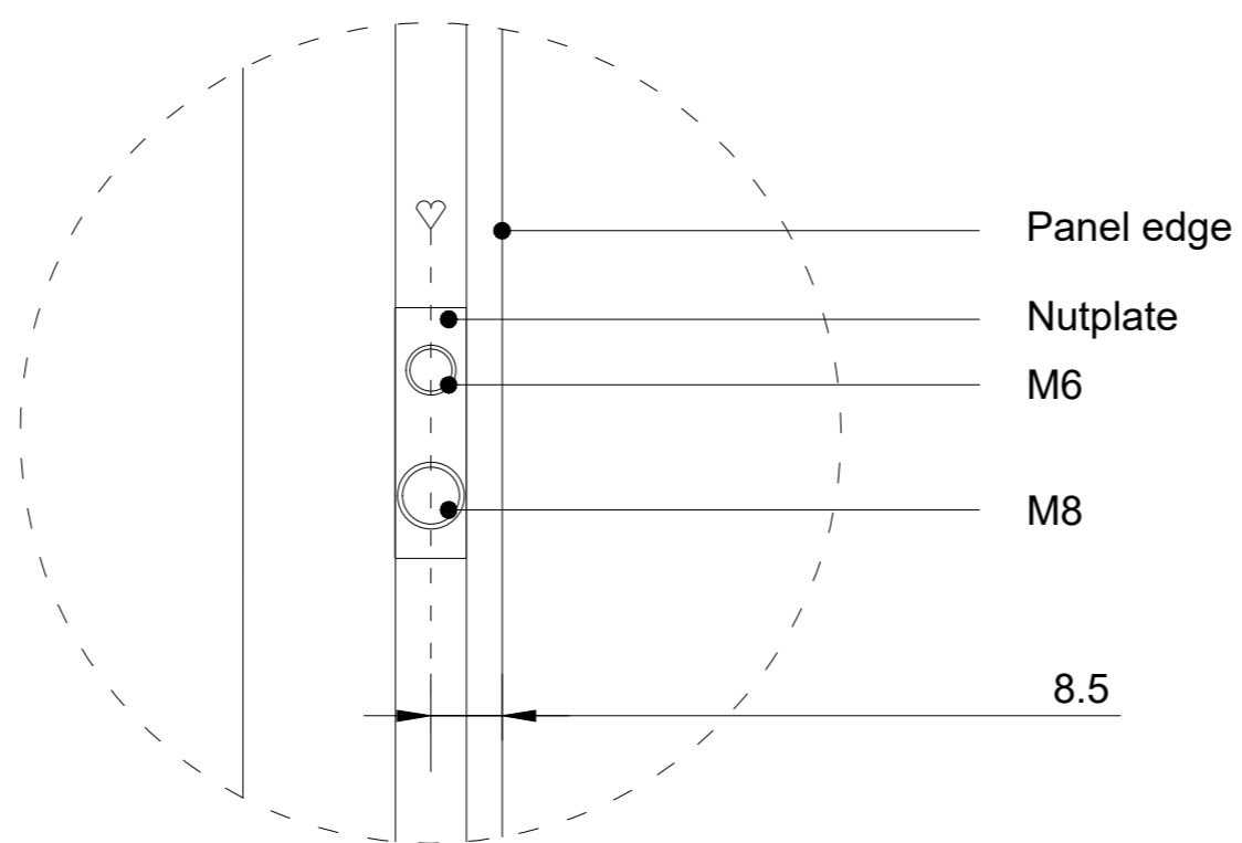
Detail 1 (1:1)
