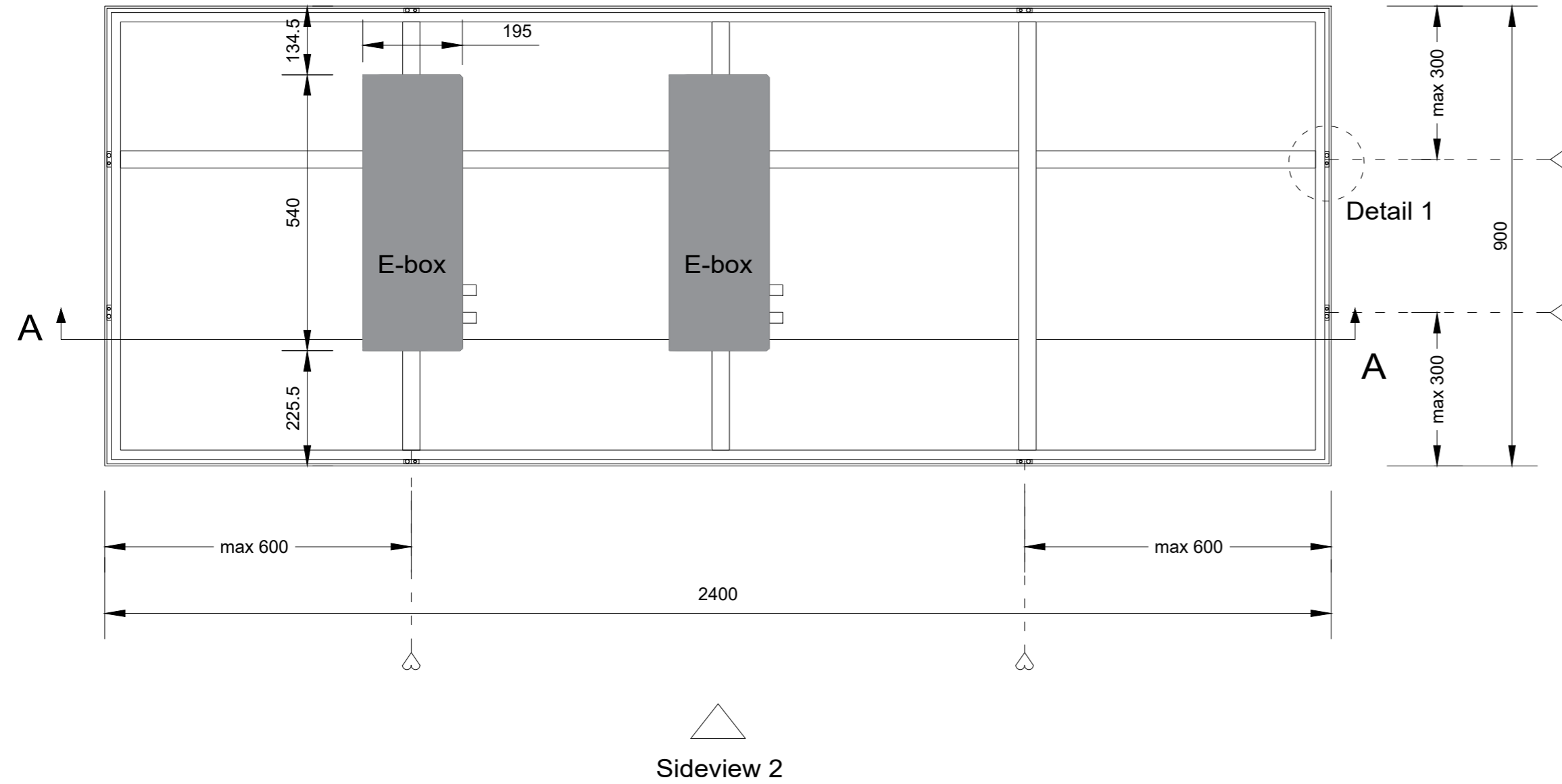
Backview (1:10)
