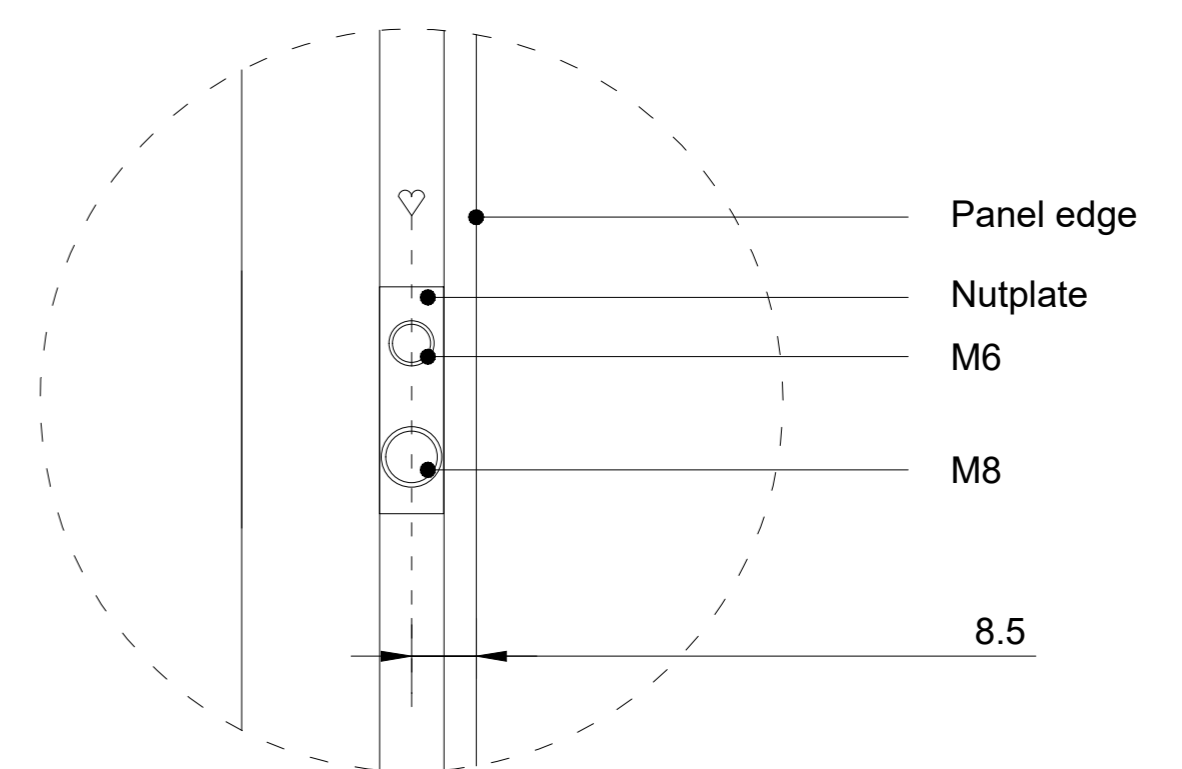
Detail 1 (1:1)
