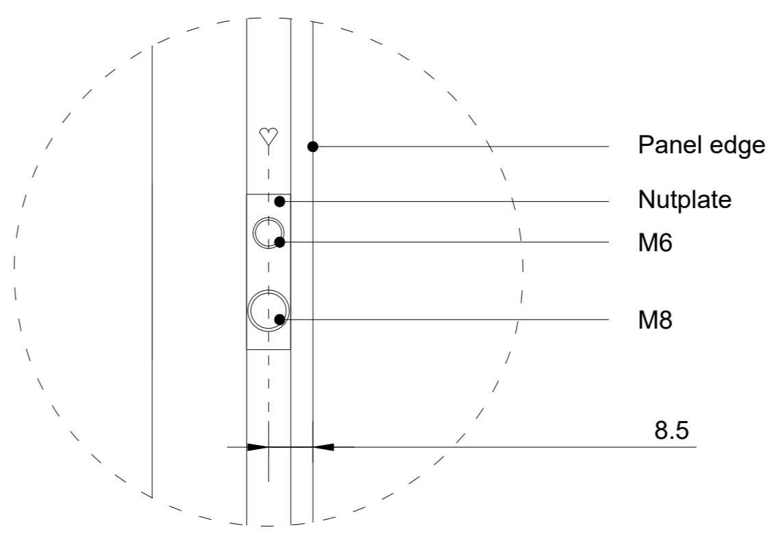
Detail 1 (1:1)
