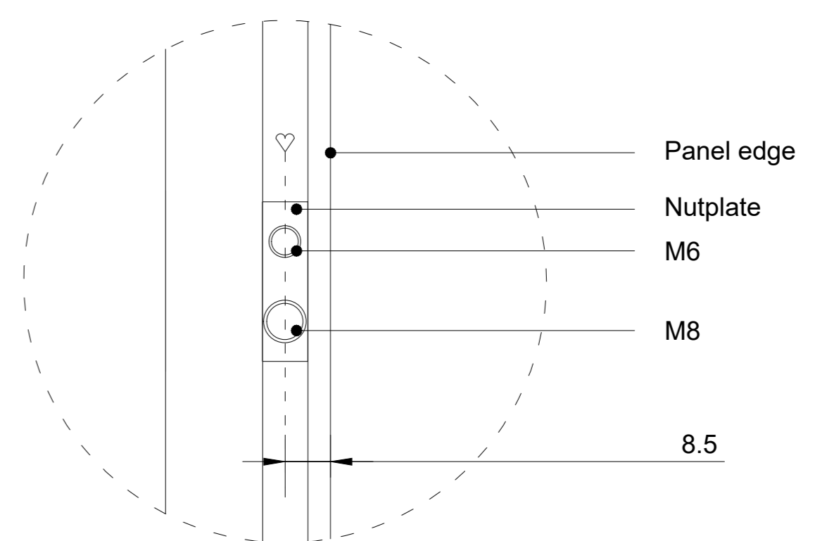
Detail 1 (1:1)
