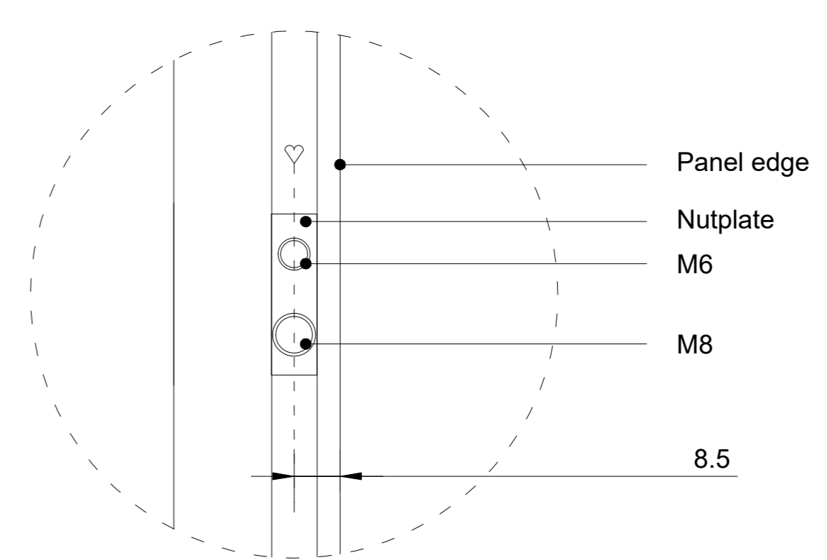
Detail 1 (1:1)
