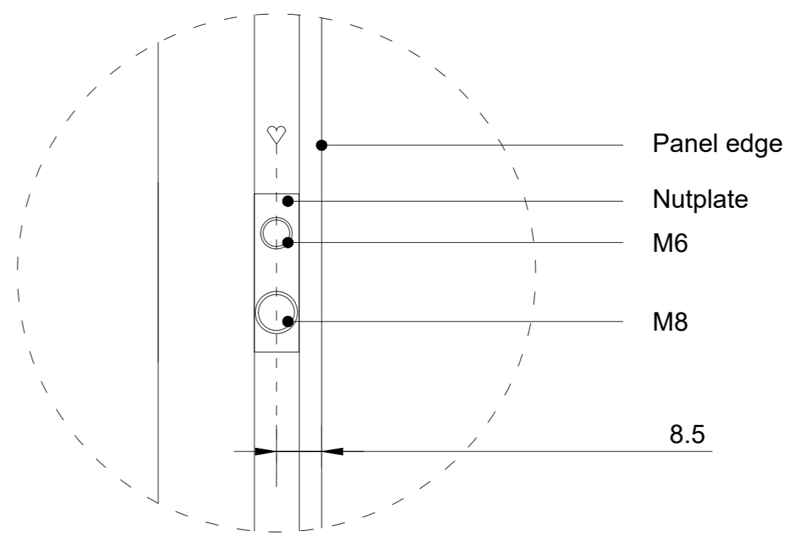
Detail 1 (1:1)
