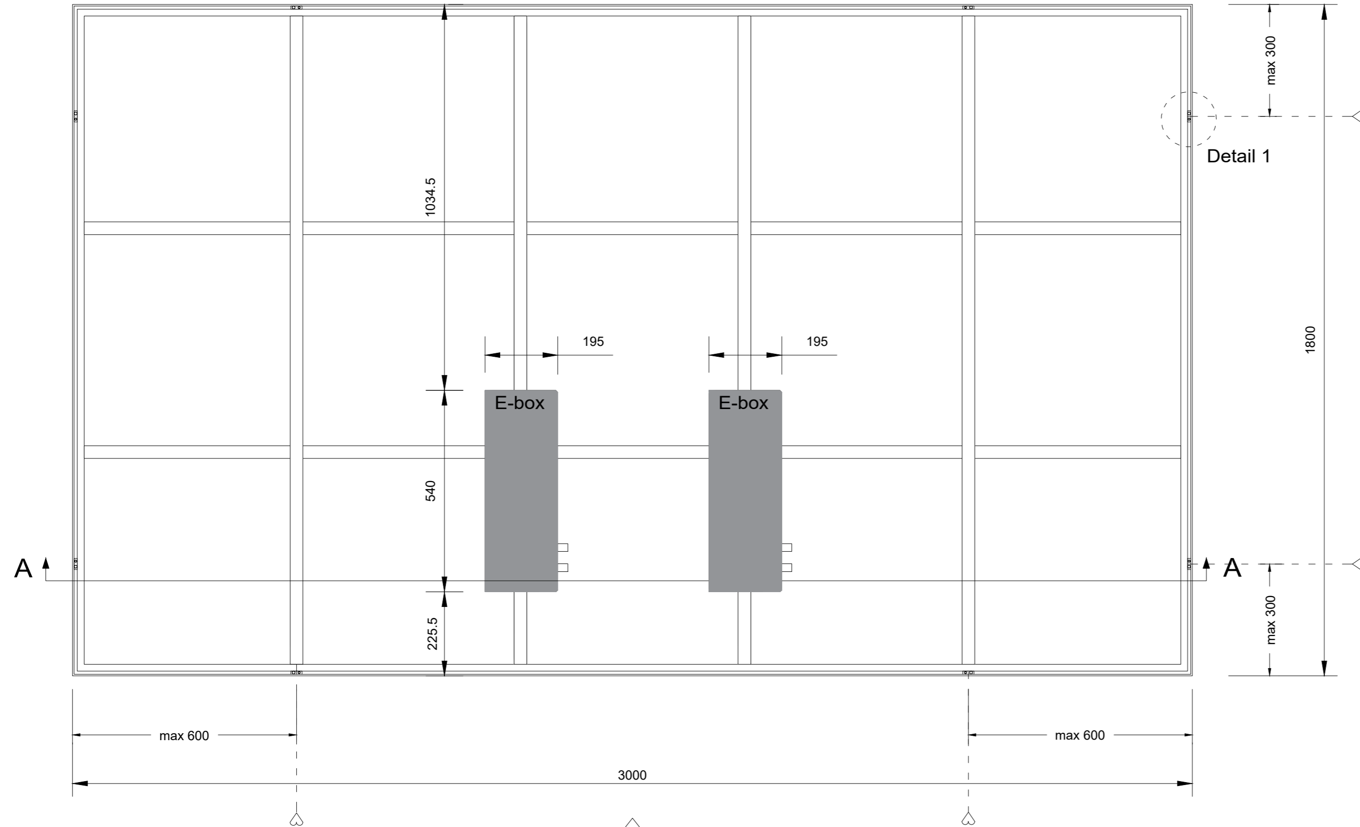
Sideview 2 - mounting position (1:10)
