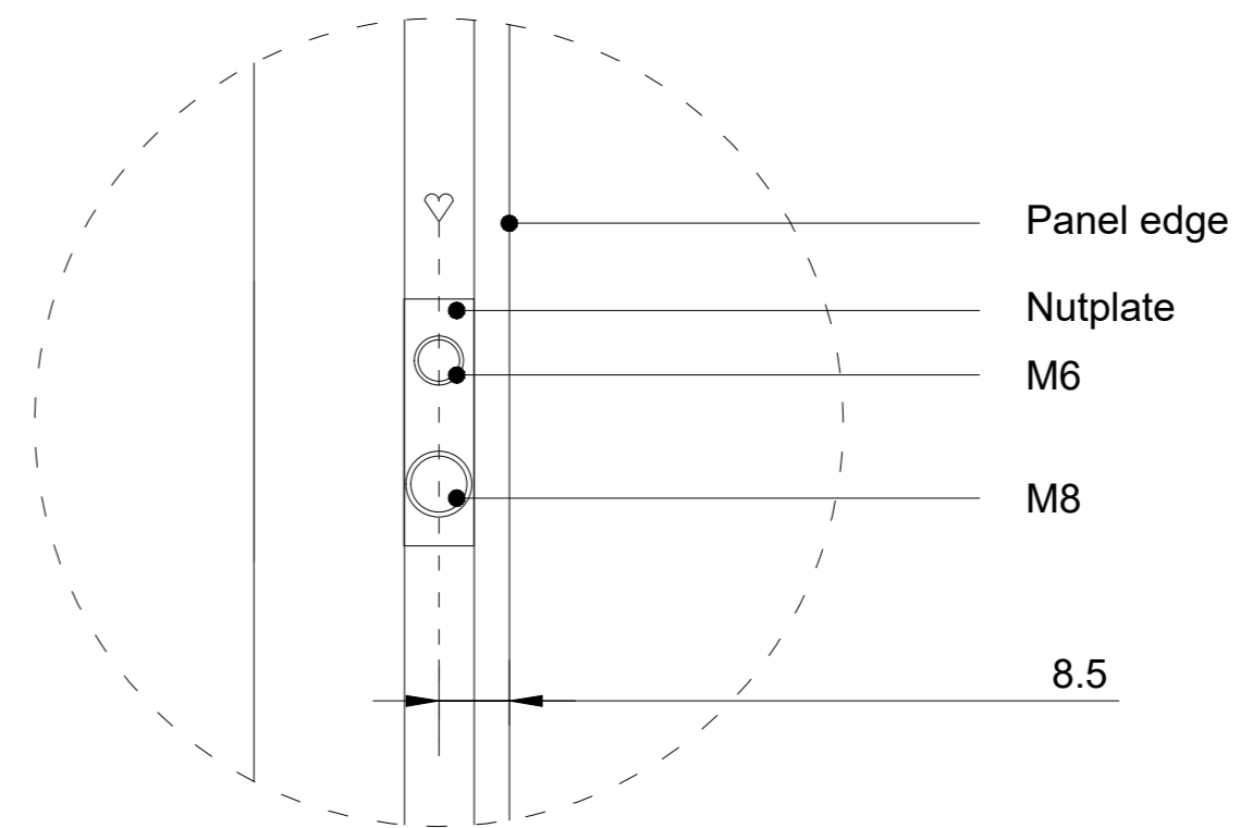
Detail 1 (1:1)
