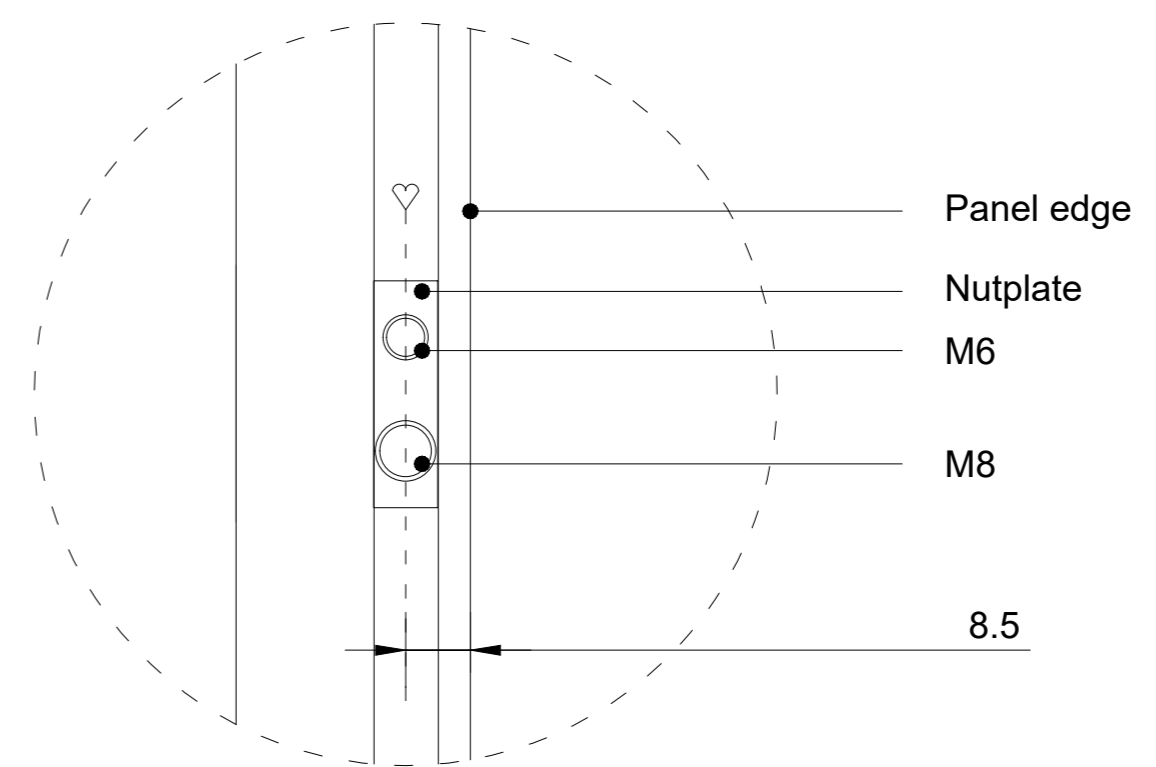
Detail 1 (1:1)
