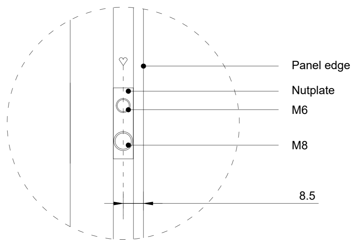
Detail 1 (1:1)
