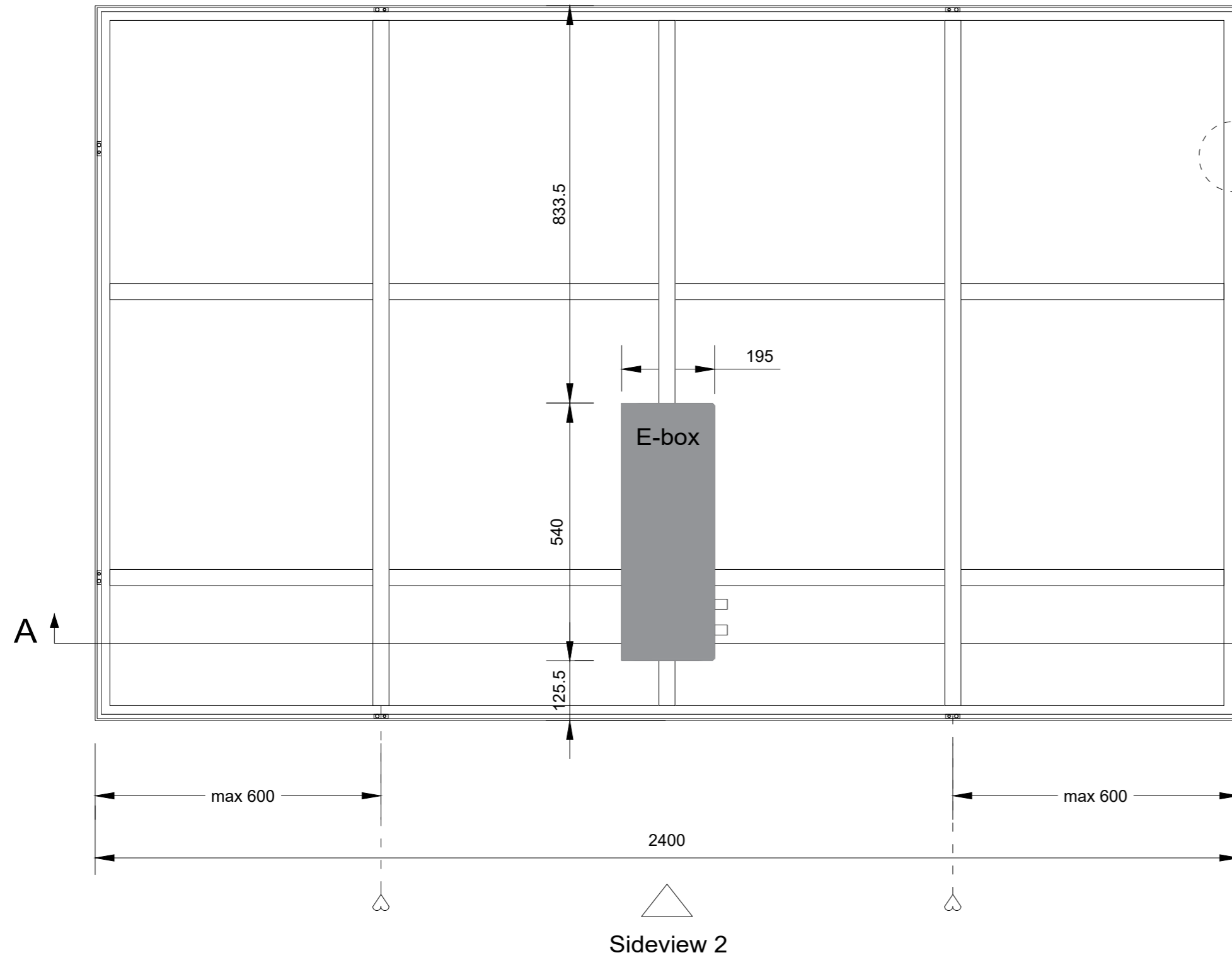
Backview (1:10)
