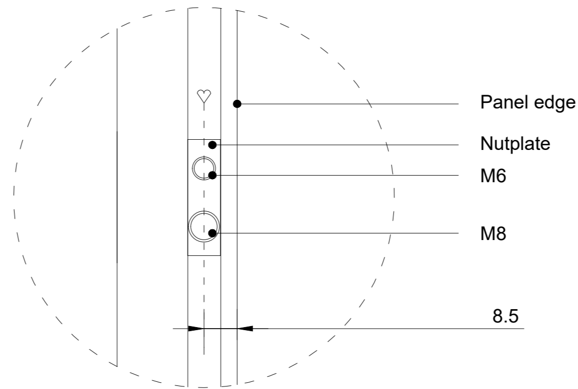
Detail 1 (1:1)
