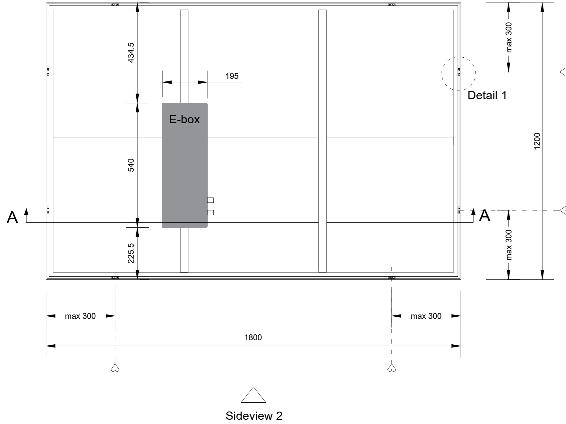
Backview (1:10)
