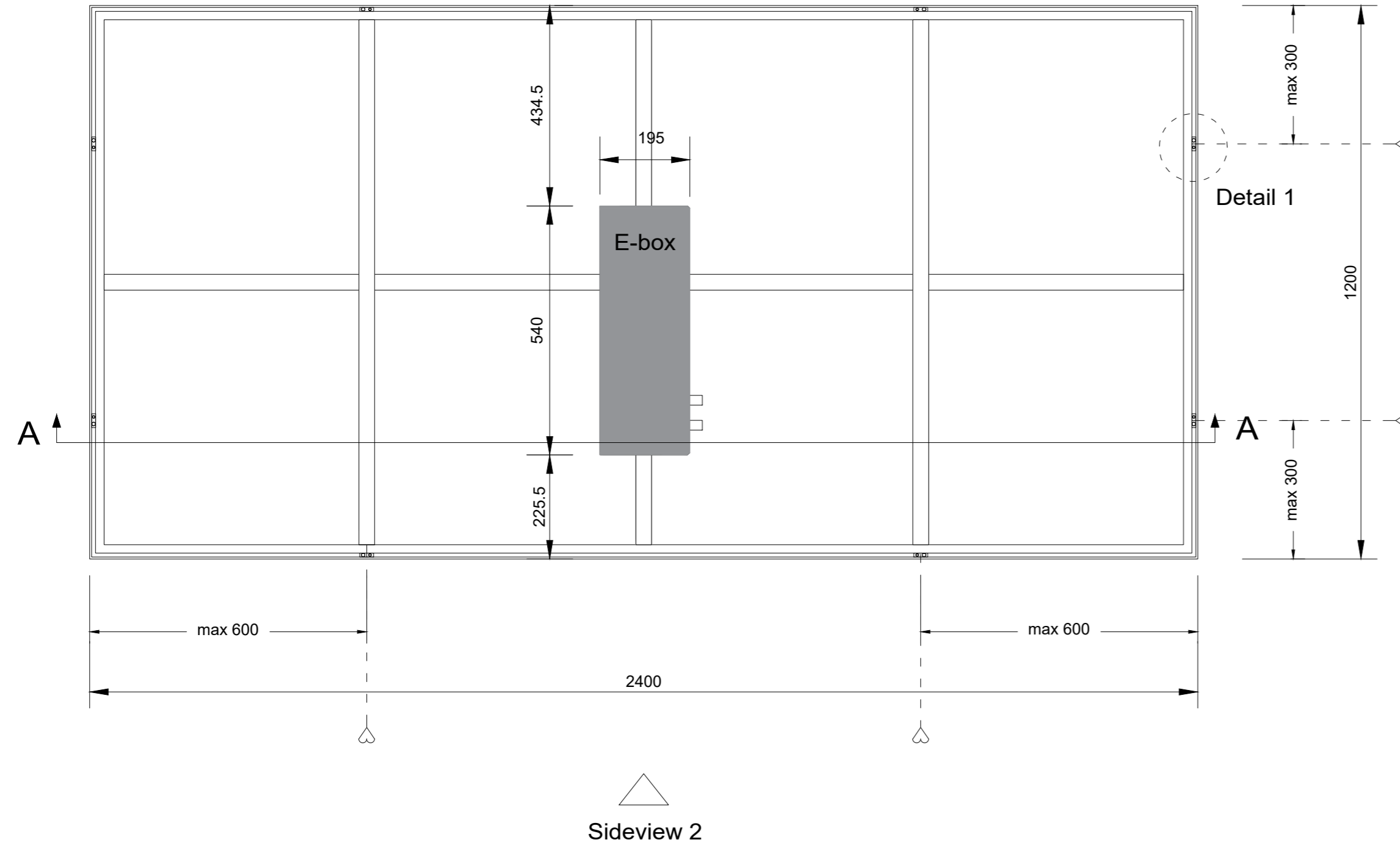
Backview (1:10)
