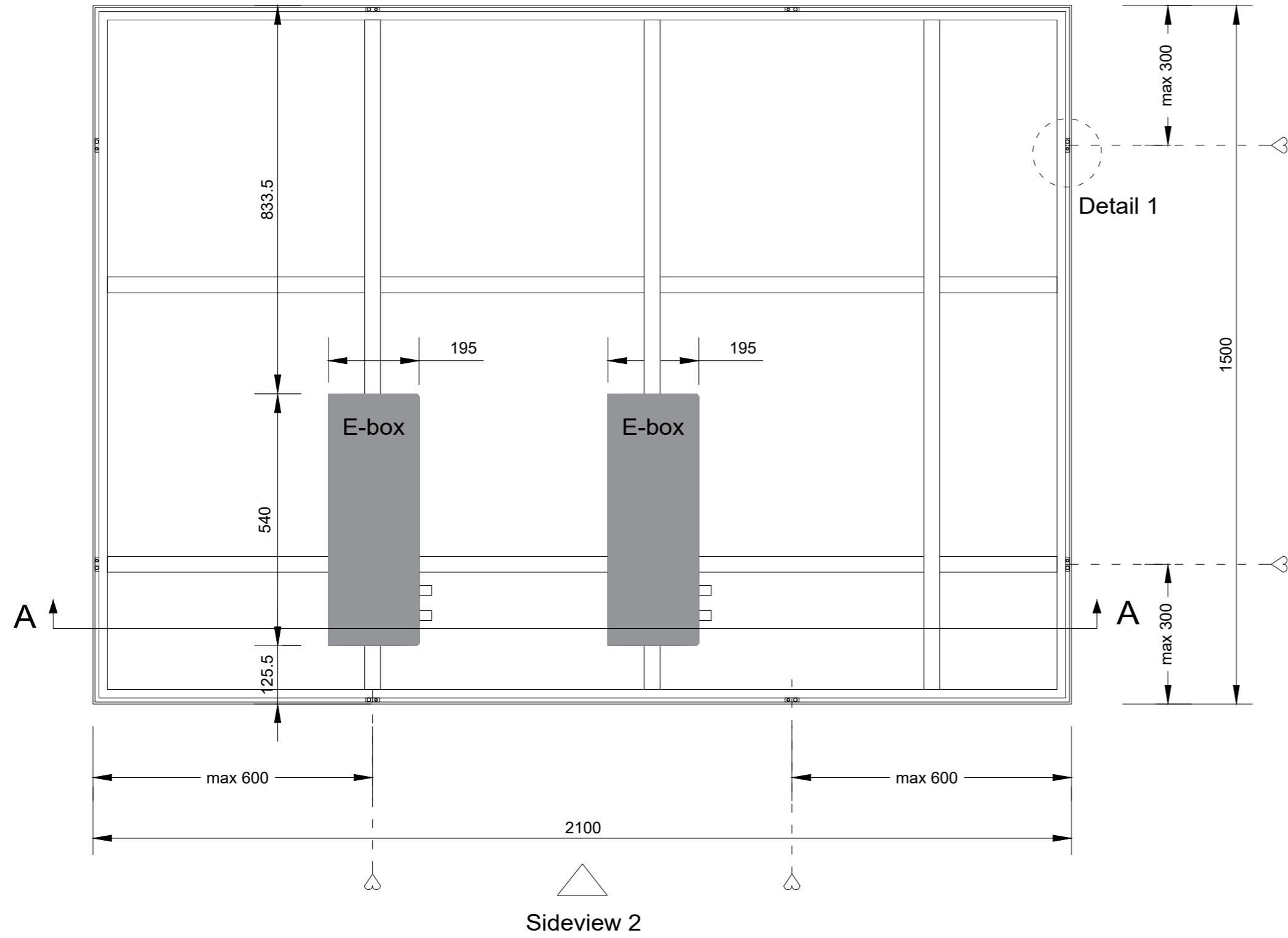
Backview (1:10)
