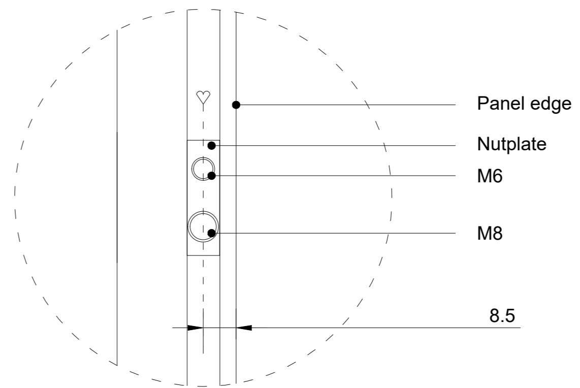
Detail 1 (1:1)
