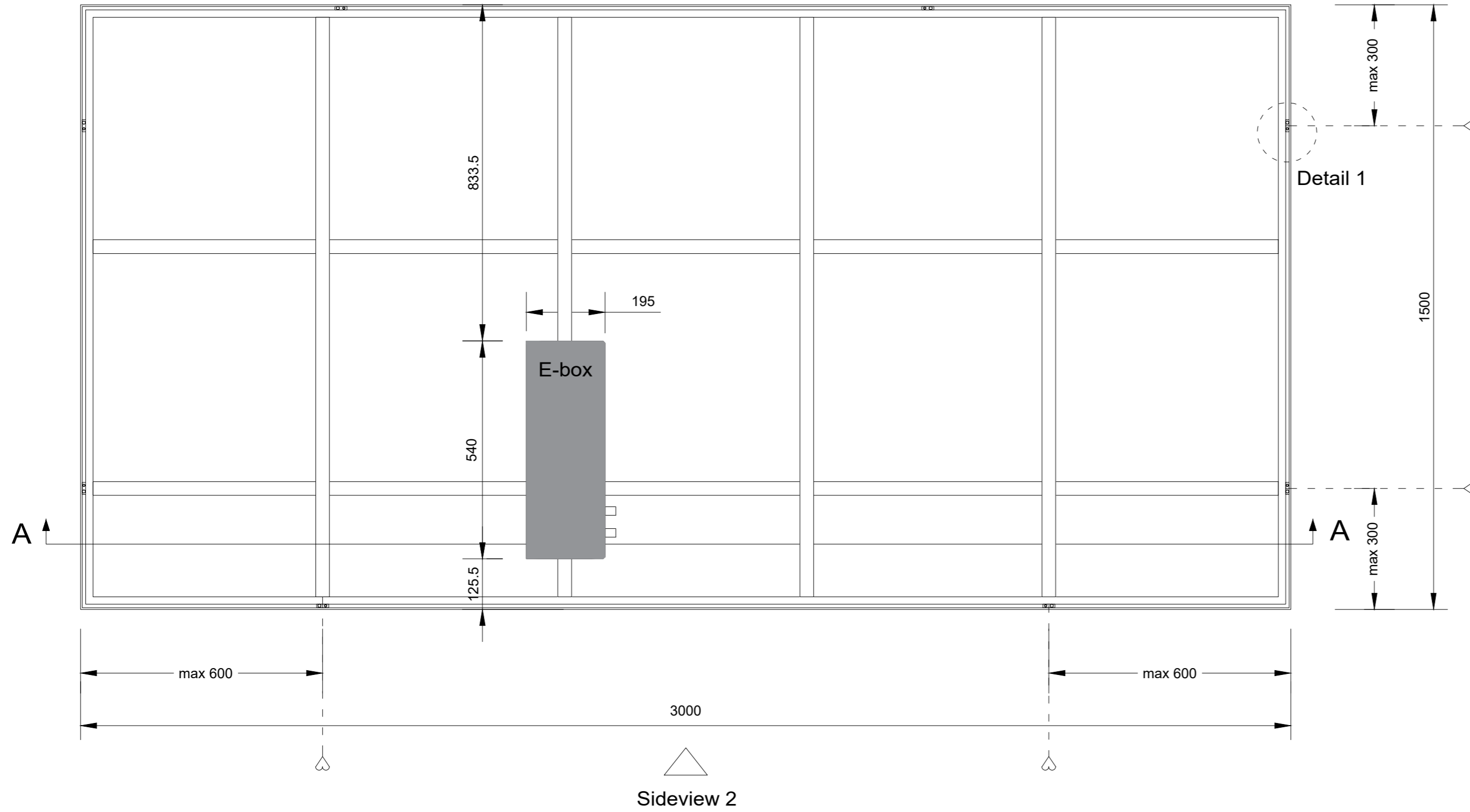
Backview (1:10)
