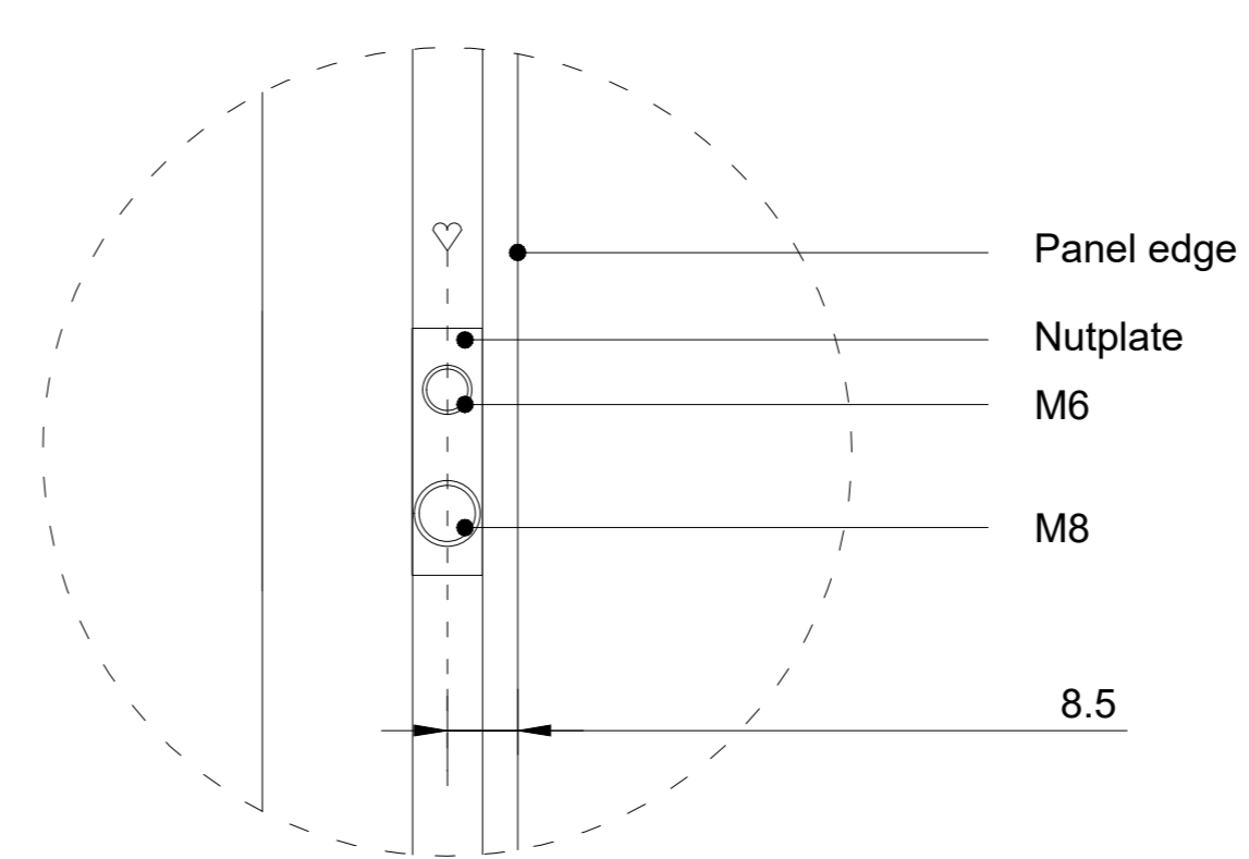
Detail 1 (1:1)
