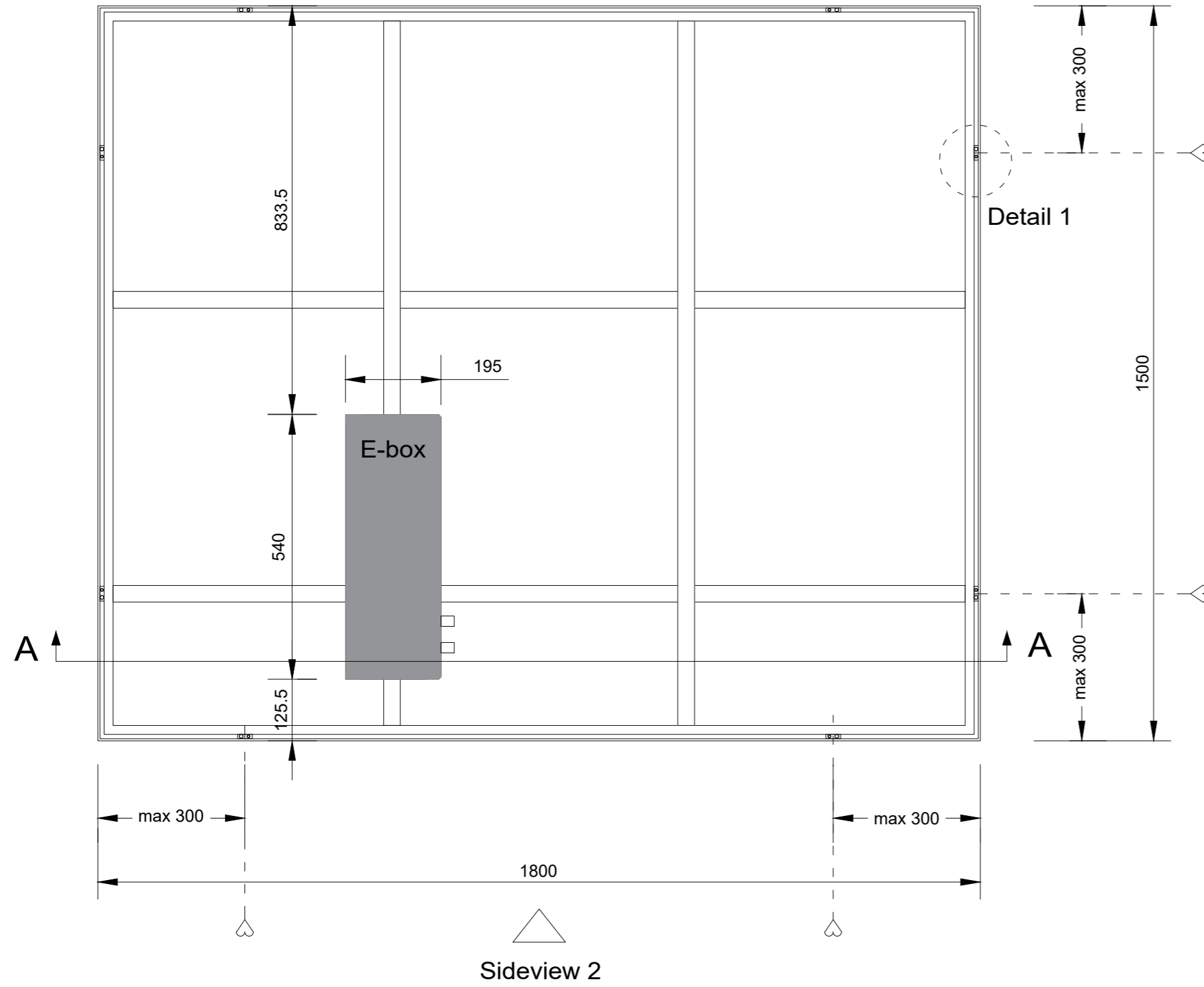
Backview (1:10)
