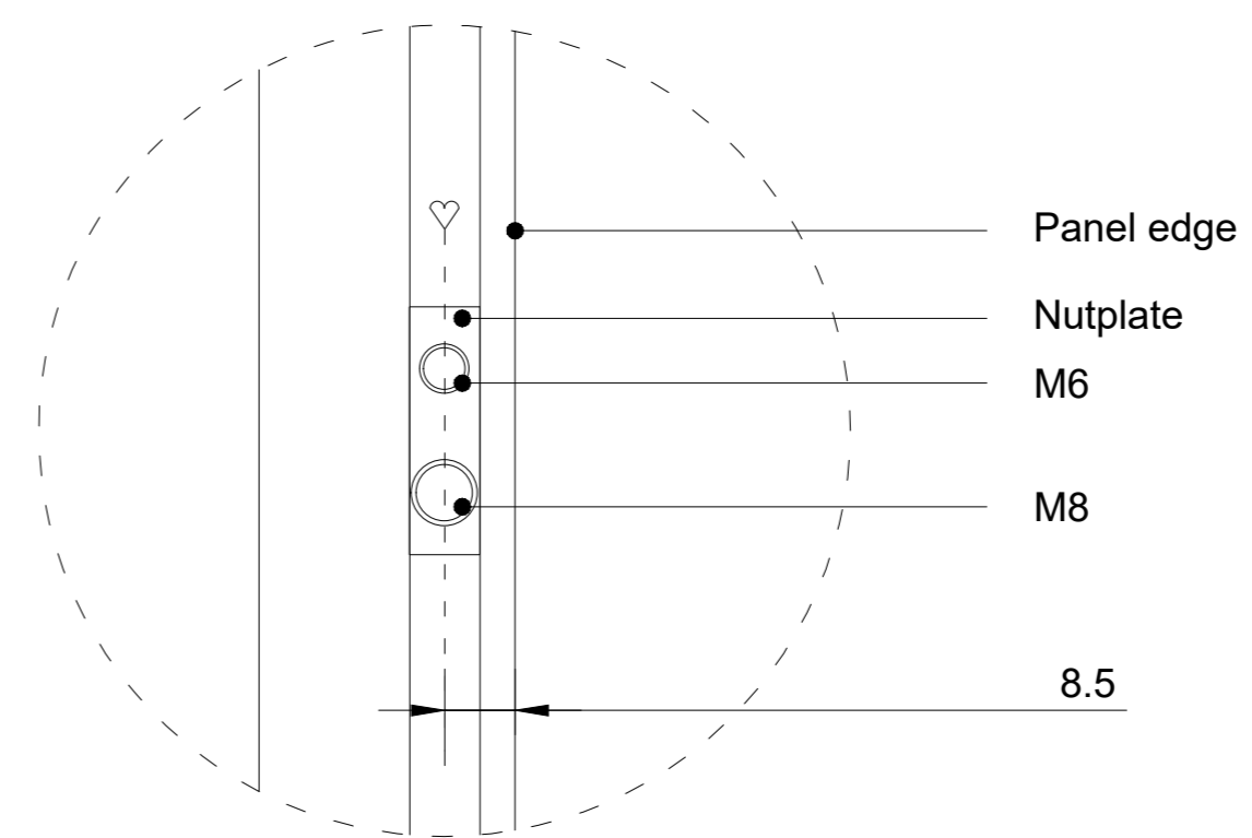
Detail 1 (1:1)
