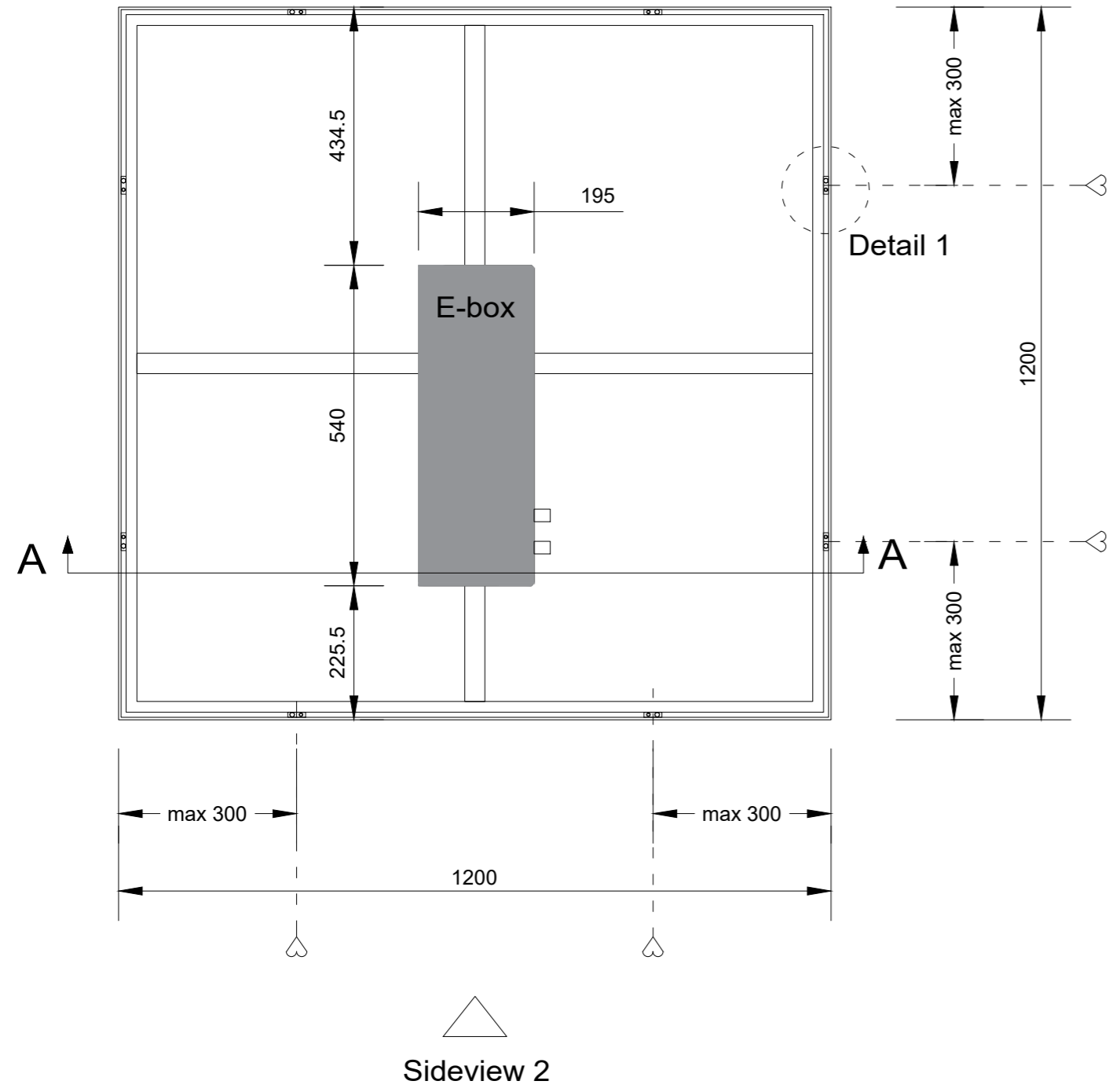
Backview (1:10)
