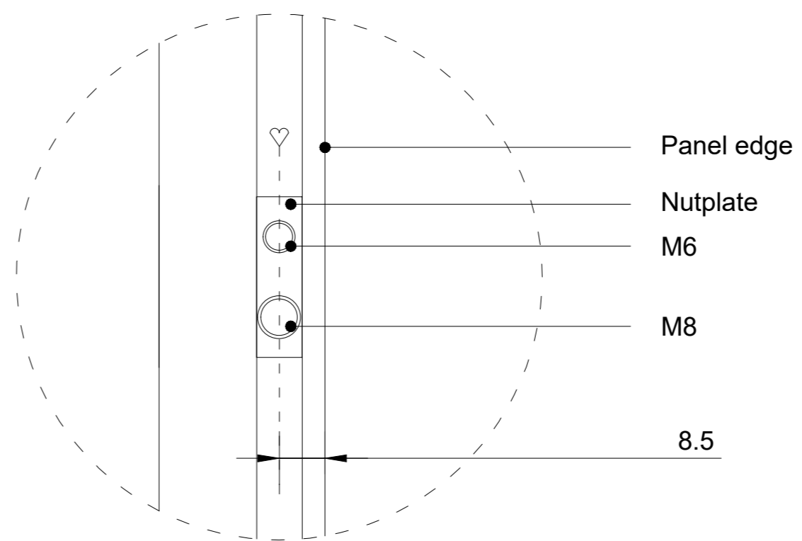
Detail 1 (1:1)
