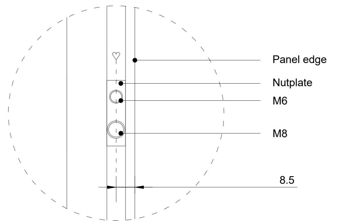
Detail 1 (1:1)
