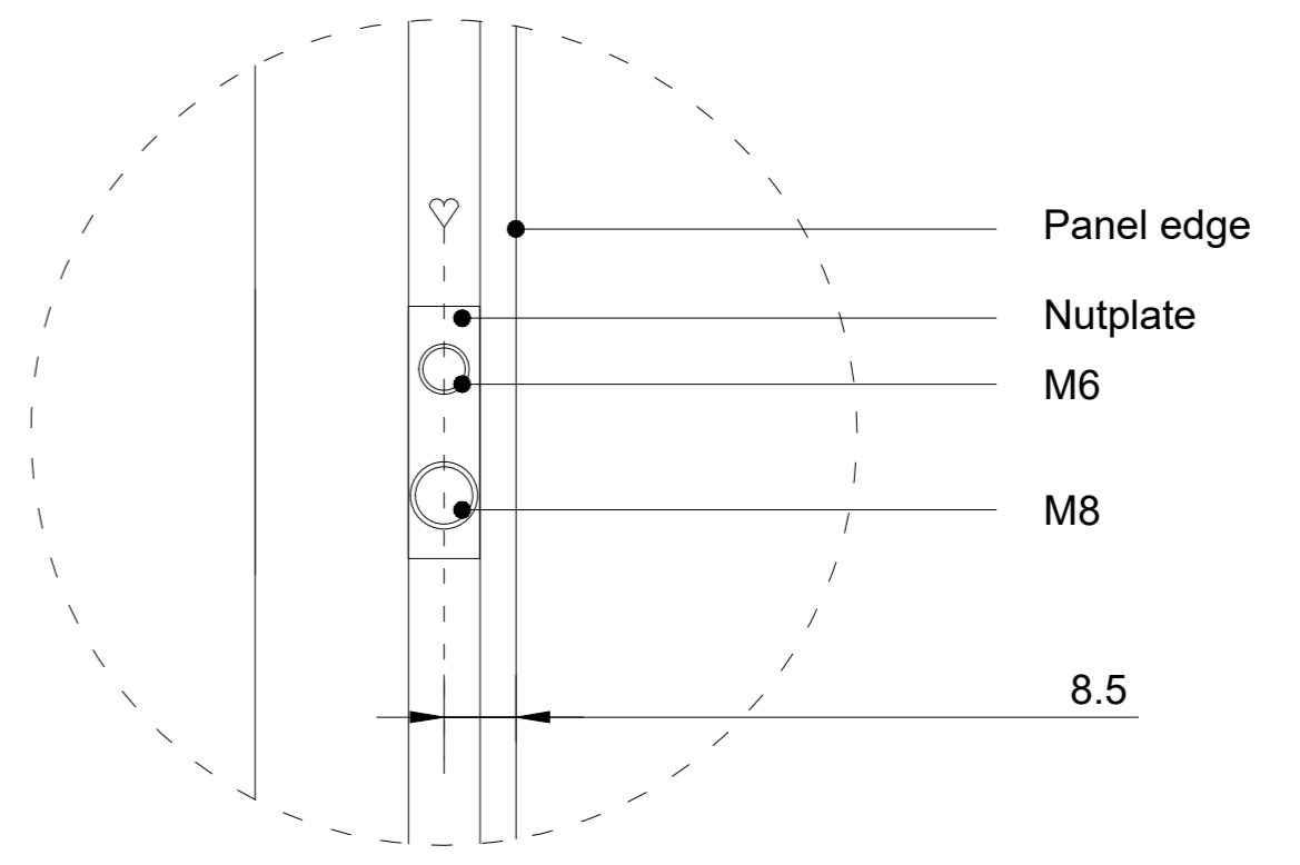
Detail 1 (1:1)
