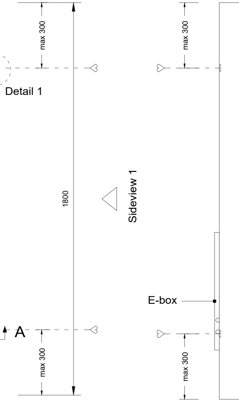
Sideview 1 - mounting position (1:10)
