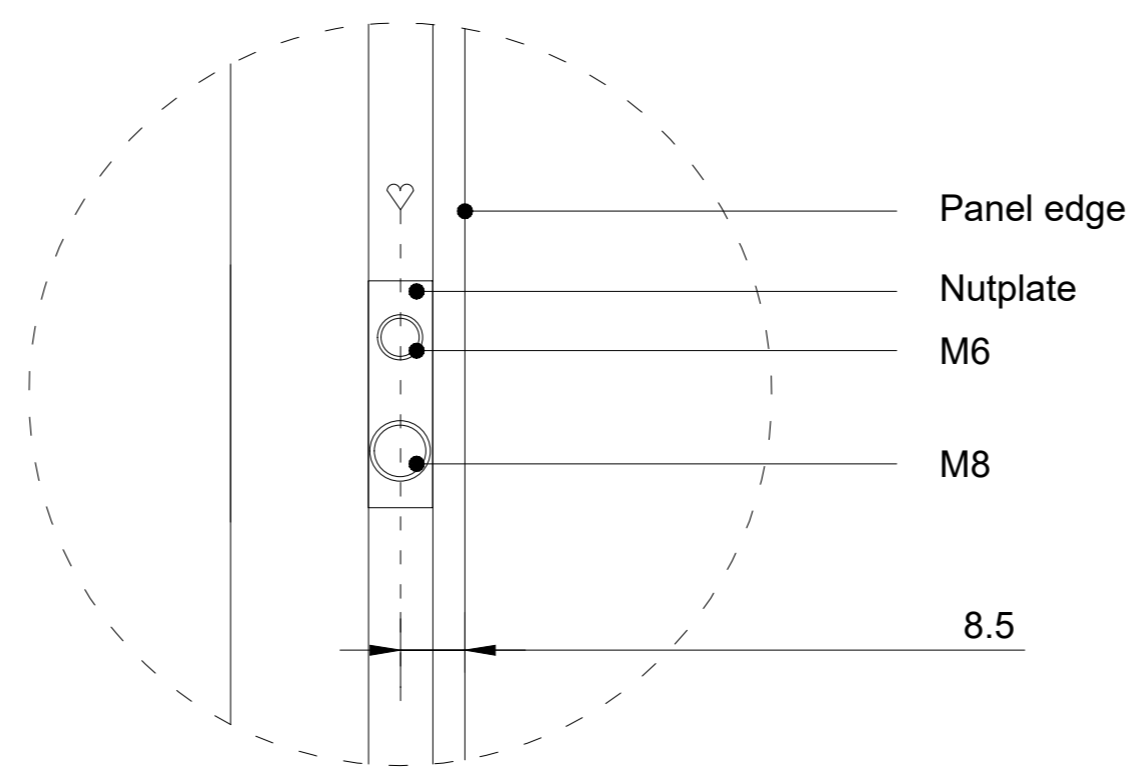
Detail 1 (1:1)
