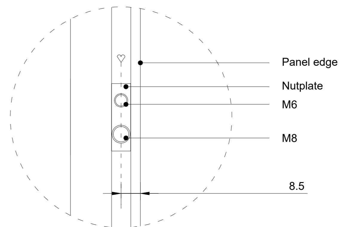
Detail 1 (1:1)
