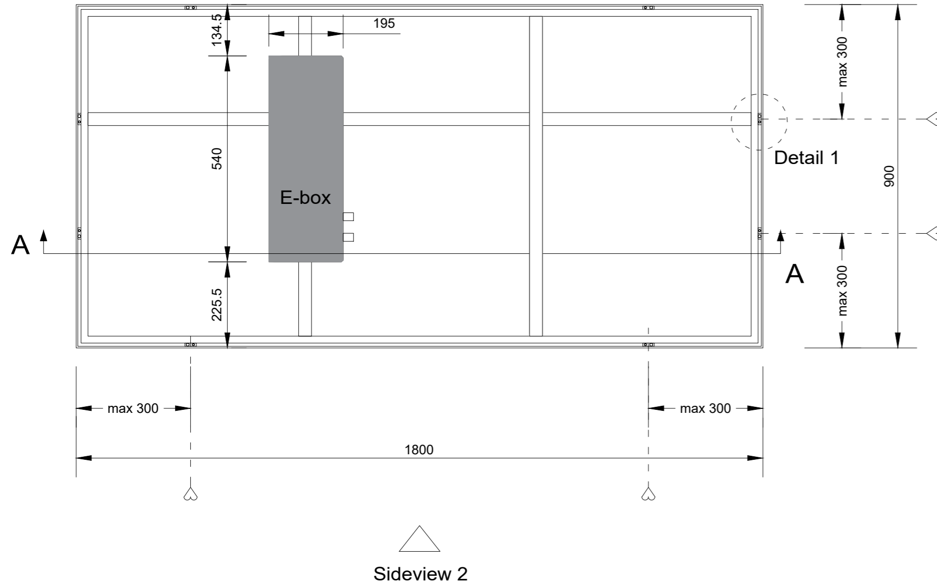
Backview (1:10)
