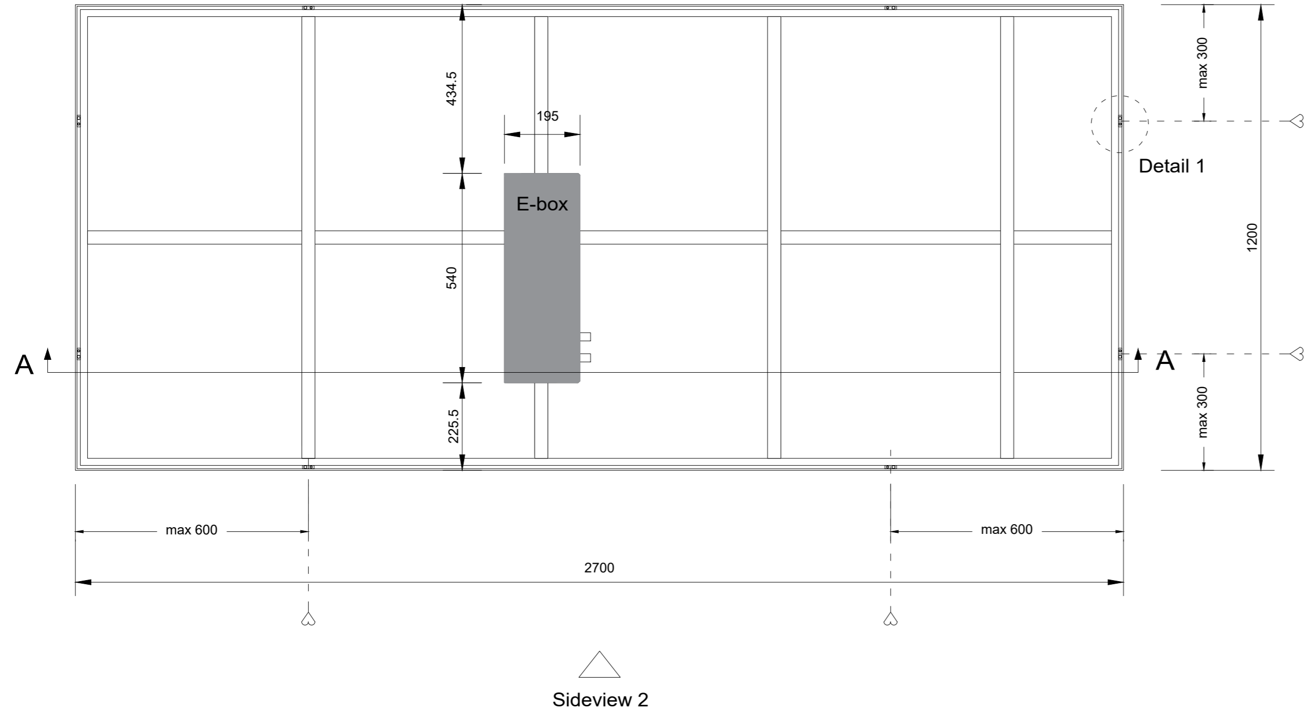
Backview (1:10)
