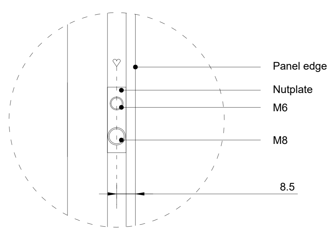
Detail 1 (1:1)
