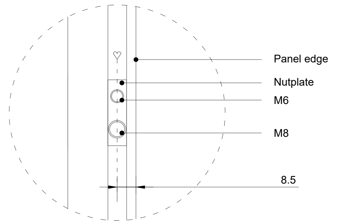
Detail 1 (1:1)
