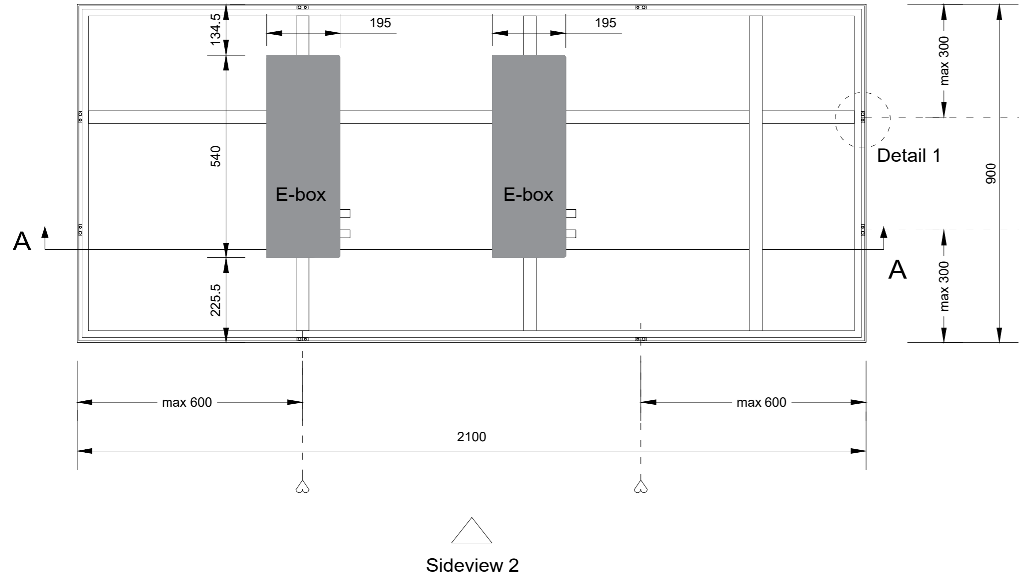
Backview (1:10)
