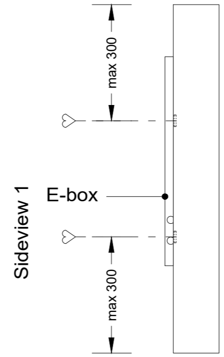
Sideview 1 - mounting position (1:10)
