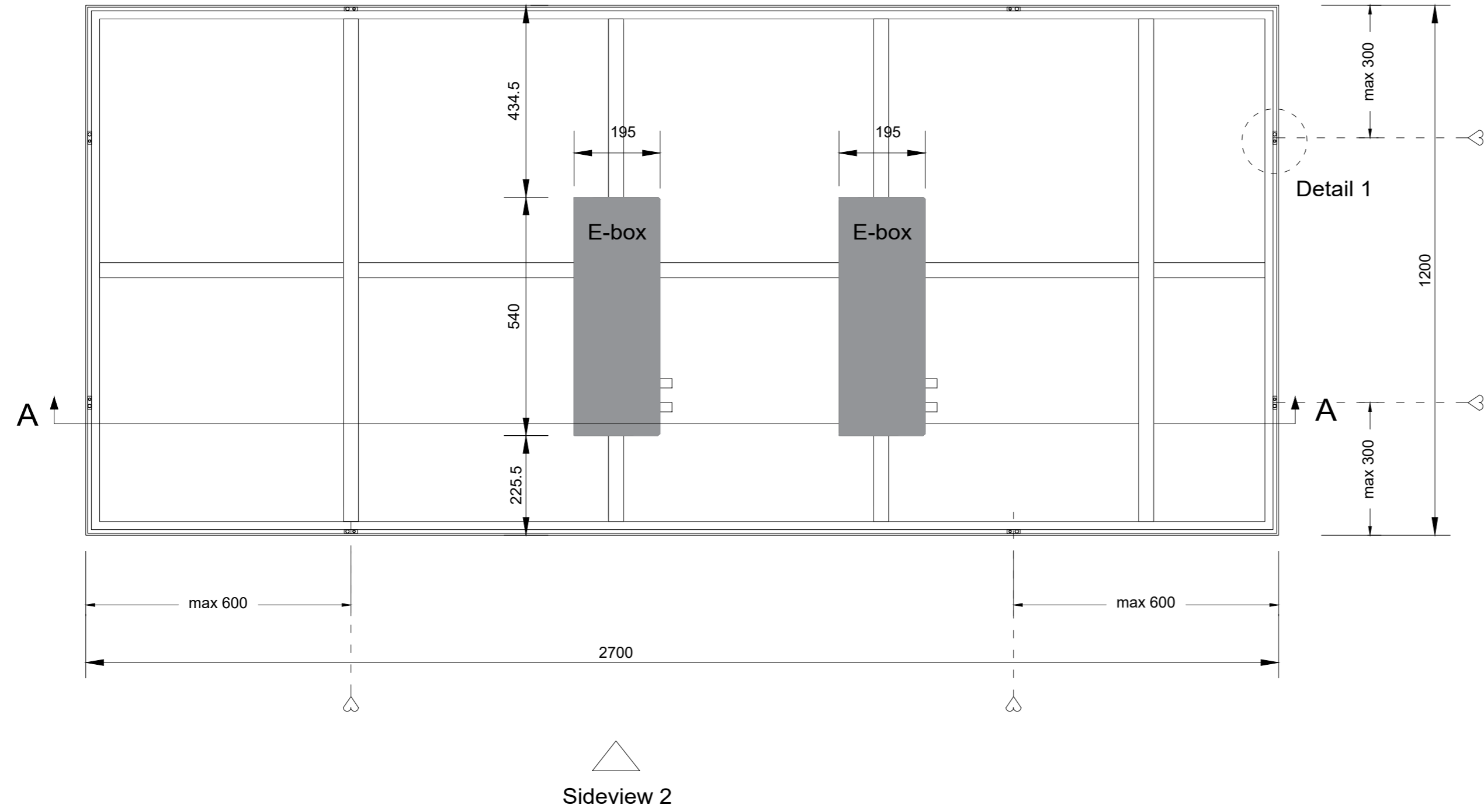
Backview (1:10)
