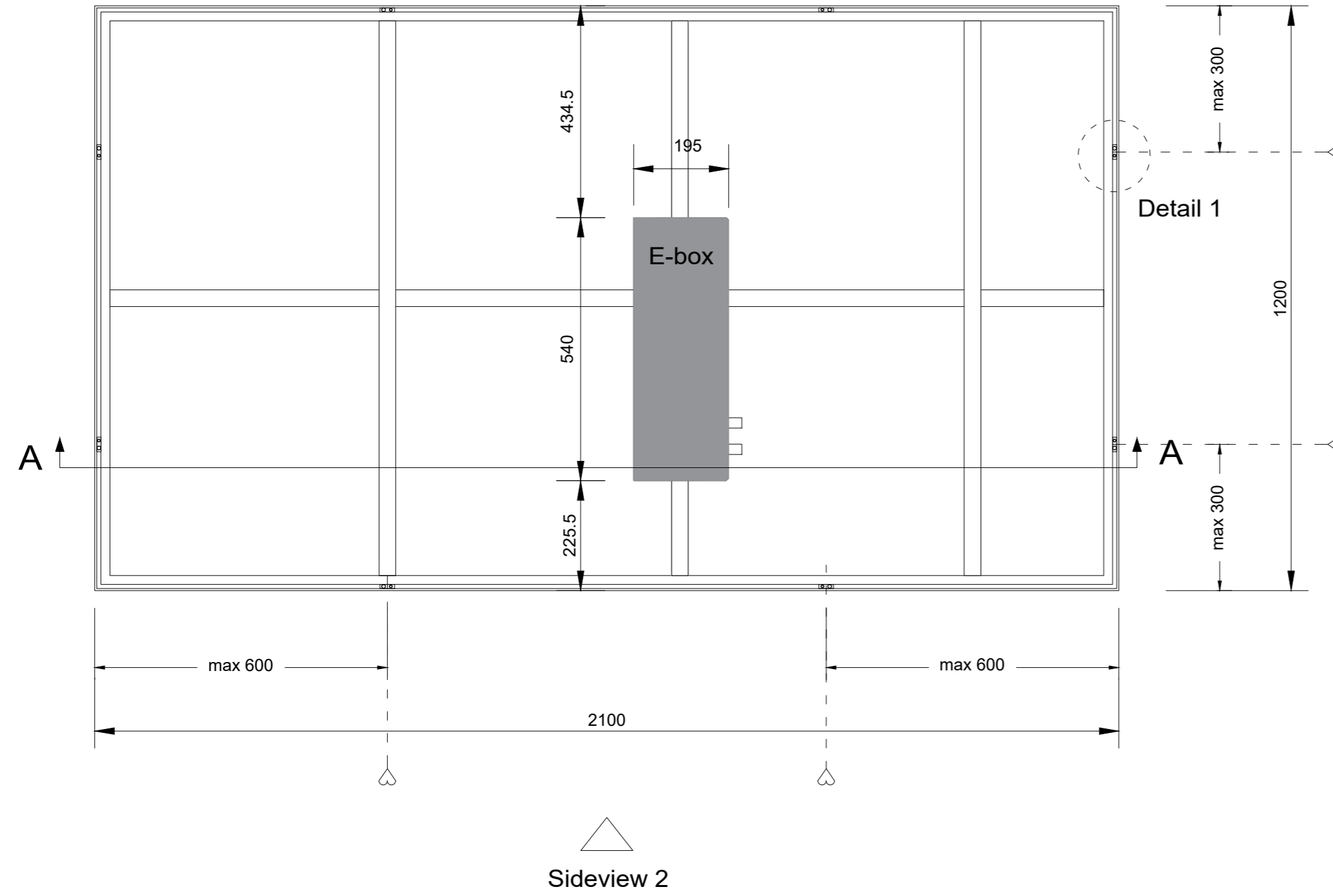
Backview (1:10)
