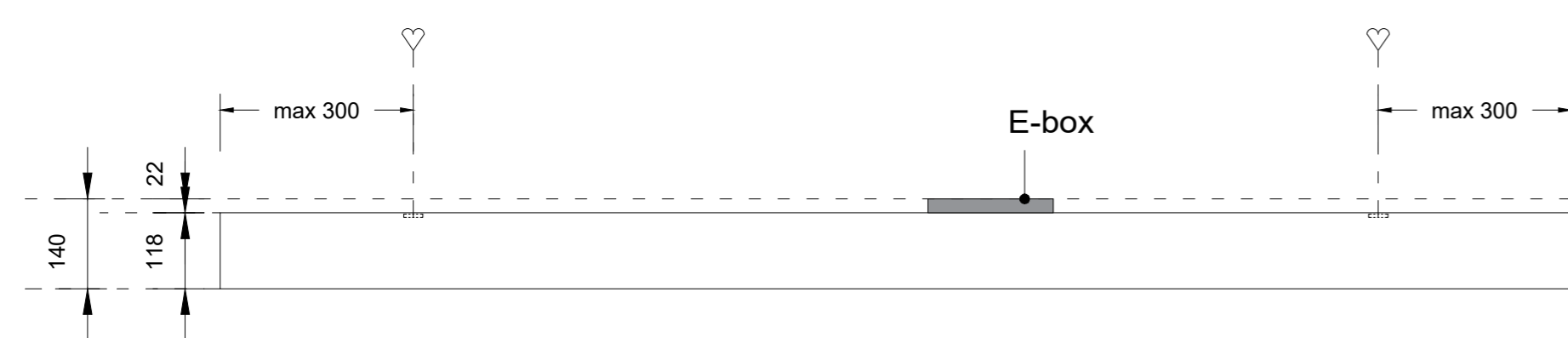
Sideview 2 - mounting position (1:10)
