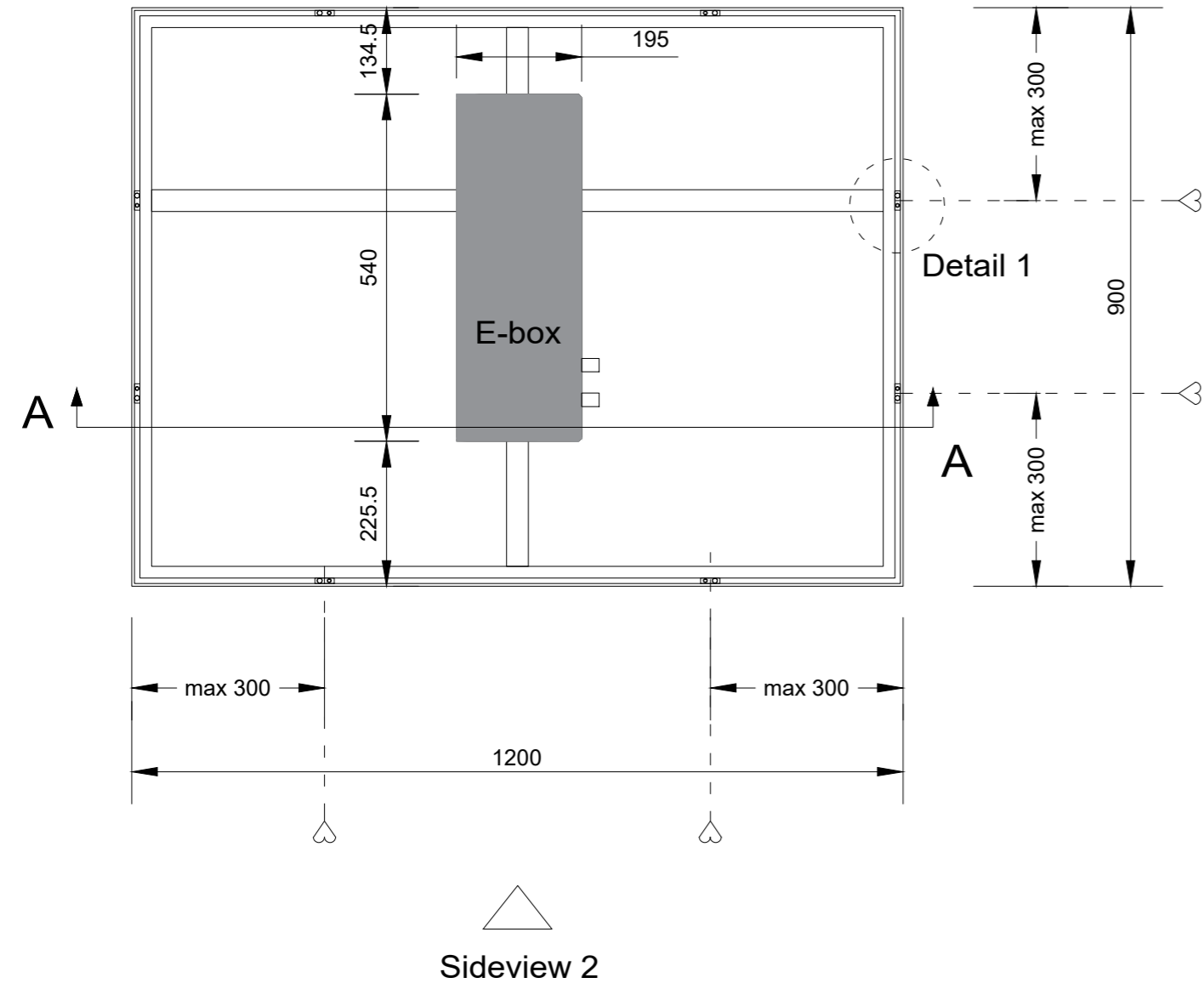
Backview (1:10)
